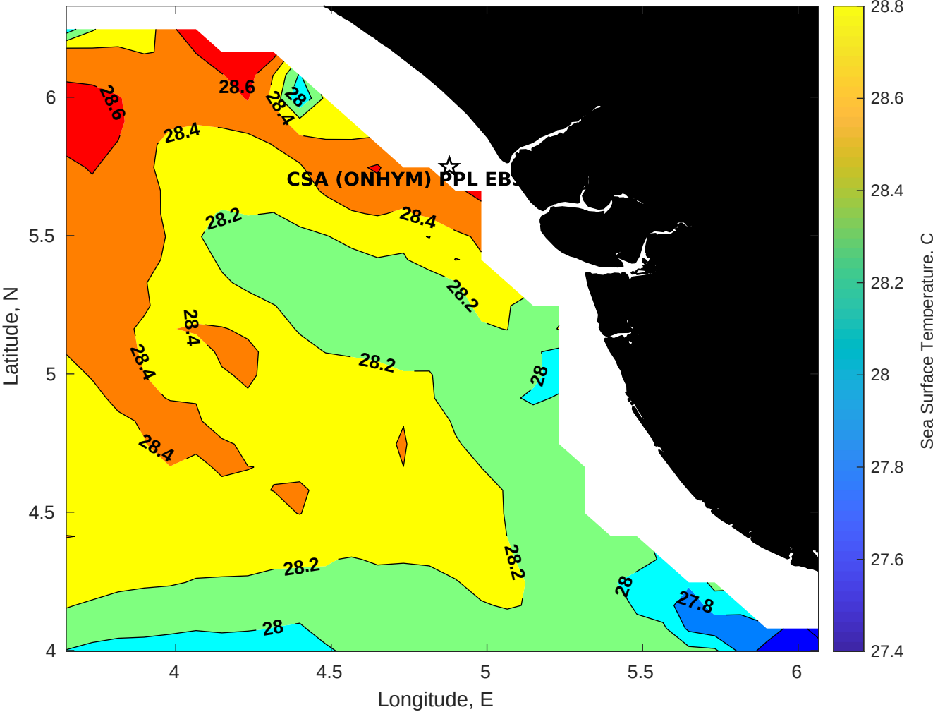
SST for CSA (ONHYM) PPL EBS - Nigeria at 11-Nov-2025 00:00:00
