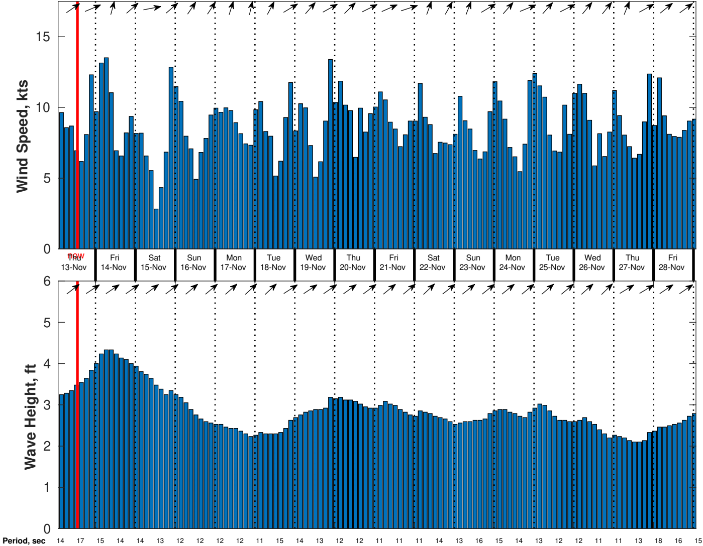
Wind & Wave Forecast for CSA (ONHYM) PPL EBS - Nigeria from 12-Nov-2025 02:00:00 to 28-Nov-2025 02:00:00
