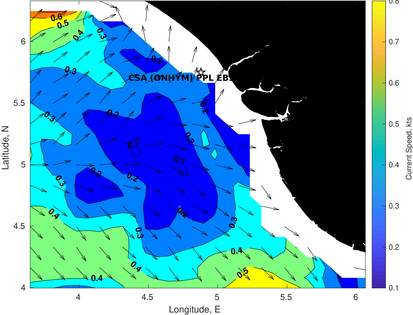
Surface Currents for CSA (ONHYM) PPL EBS - Nigeria at 11-Nov-2025 00:00:00
