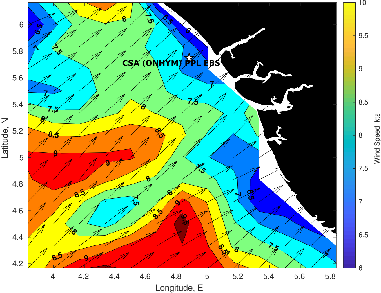
Winds (kts) for CSA (ONHYM) PPL EBS - Nigeria at 12-Nov-2025 09:00:00
