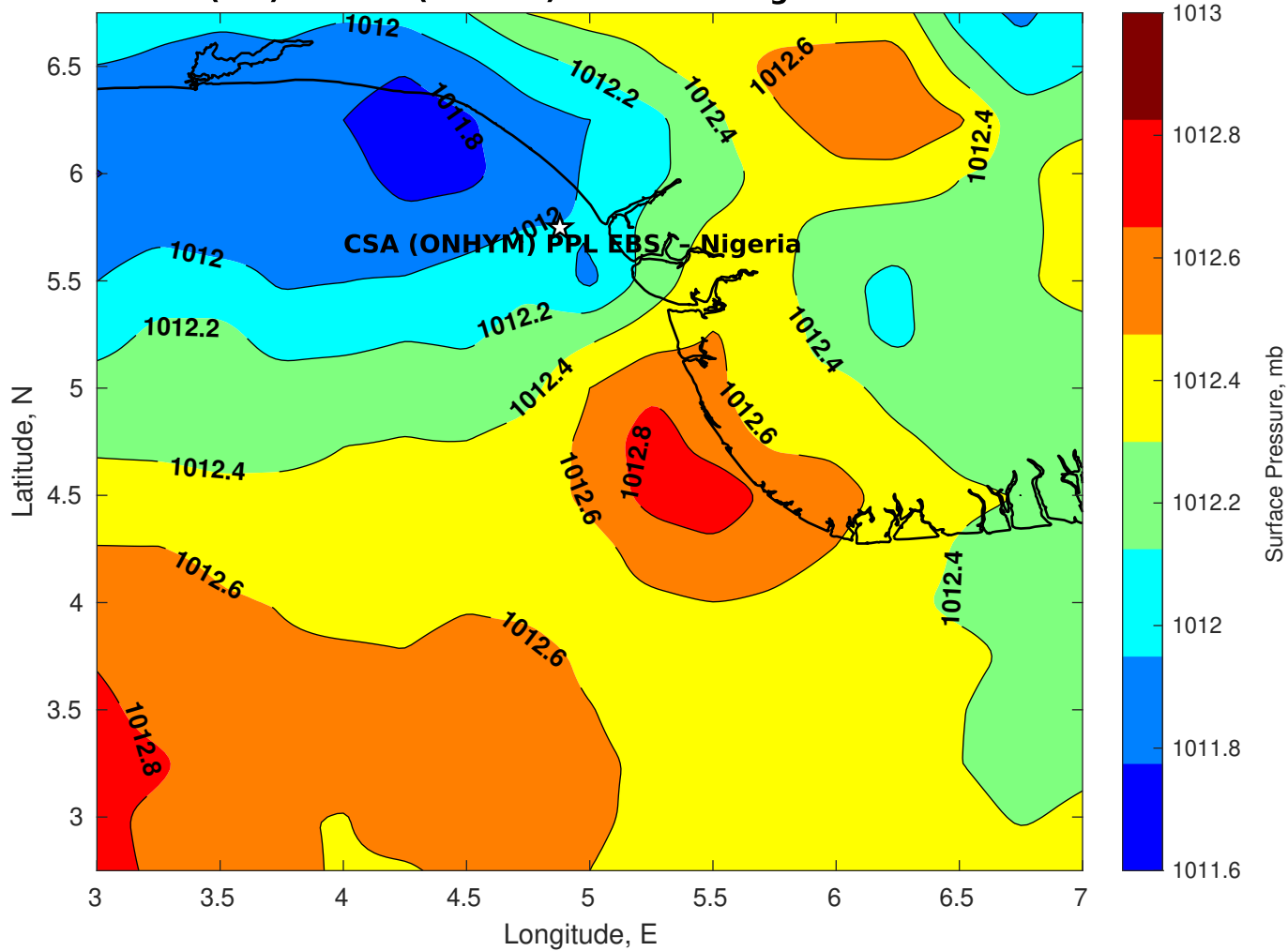
Surface Pressure (mb) for CSA (ONHYM) PPL EBS - Nigeria at 13-Nov-2025 00:00:00
