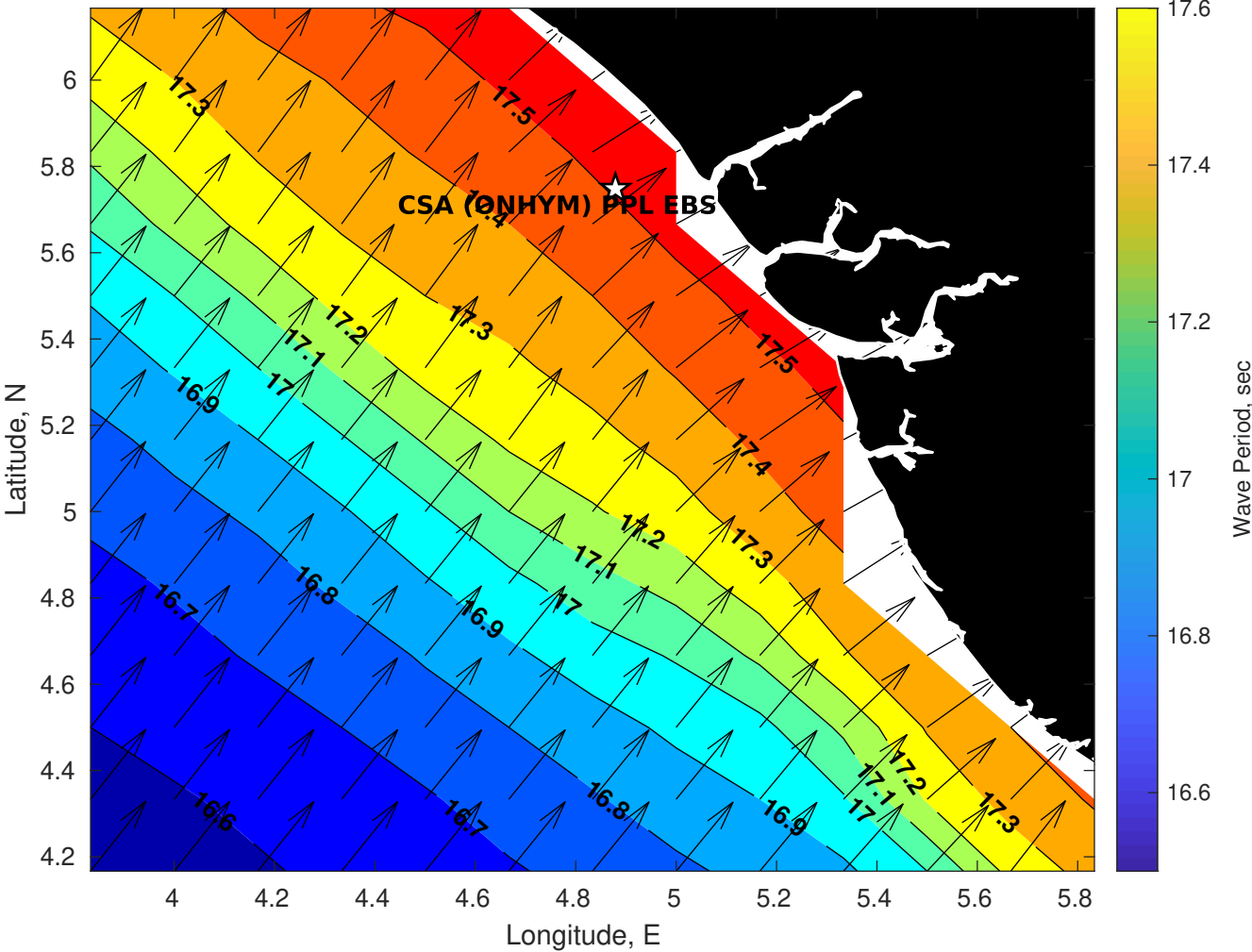
Wave Period (sec) for CSA (ONHYM) PPL EBS - Nigeria at 12-Nov-2025 09:00:00
