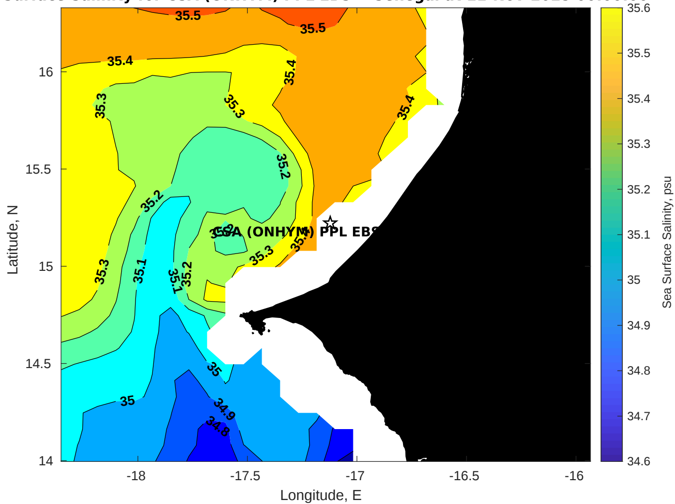
Surface Salinity for CSA (ONHYM) PPL EBS - Senegal at 11-Nov-2025 00:00:00
