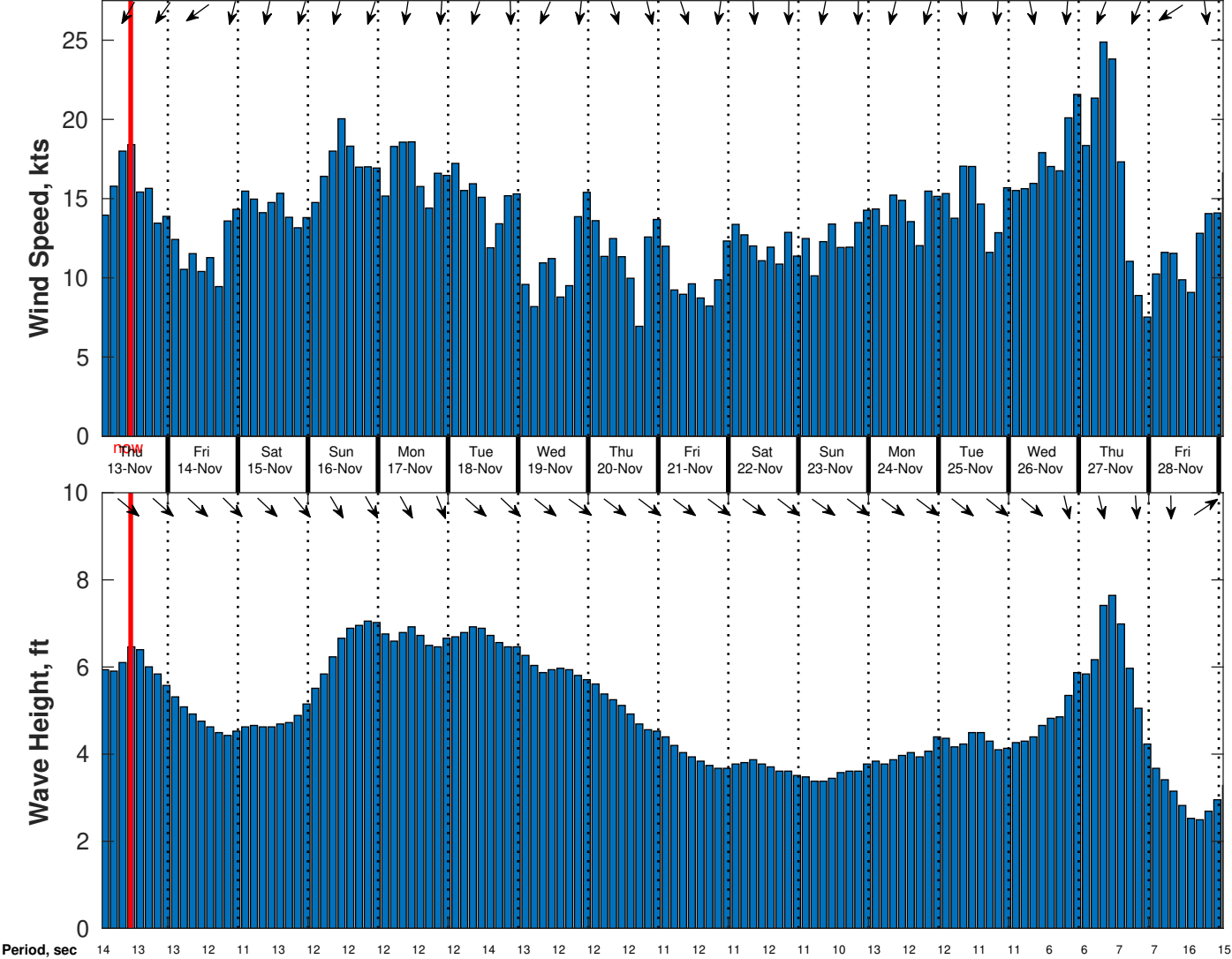
Wind & Wave Forecast for CSA (ONHYM) PPL EBS - Senegal from 12-Nov-2025 01:00:00 to 28-Nov-2025 01:00:00
