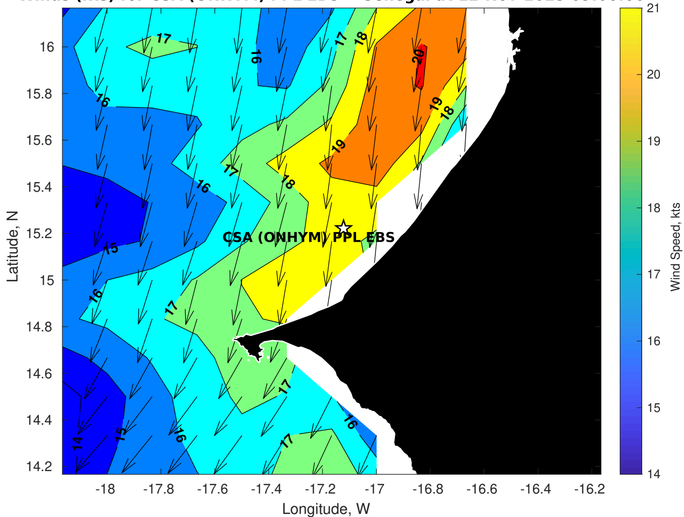
Winds (kts) for CSA (ONHYM) PPL EBS - Senegal at 12-Nov-2025 09:00:00
