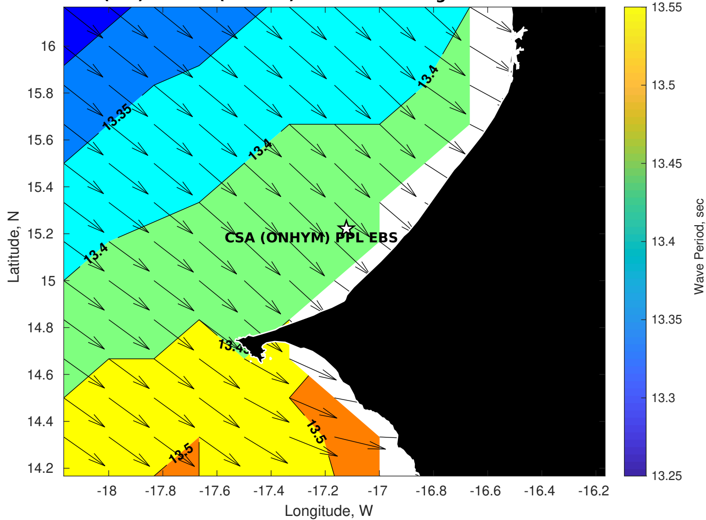
Wave Period (sec) for CSA (ONHYM) PPL EBS - Senegal at 12-Nov-2025 09:00:00
