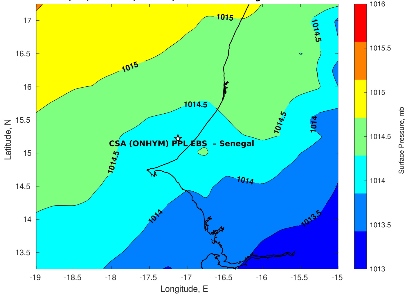
Surface Pressure (mb) for CSA (ONHYM) PPL EBS - Senegal at 13-Nov-2025 00:00:00
