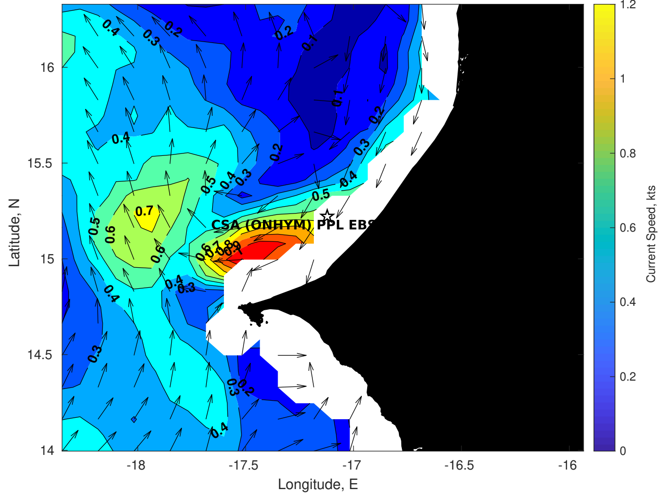
Surface Currents for CSA (ONHYM) PPL EBS - Senegal at 11-Nov-2025 00:00:00
