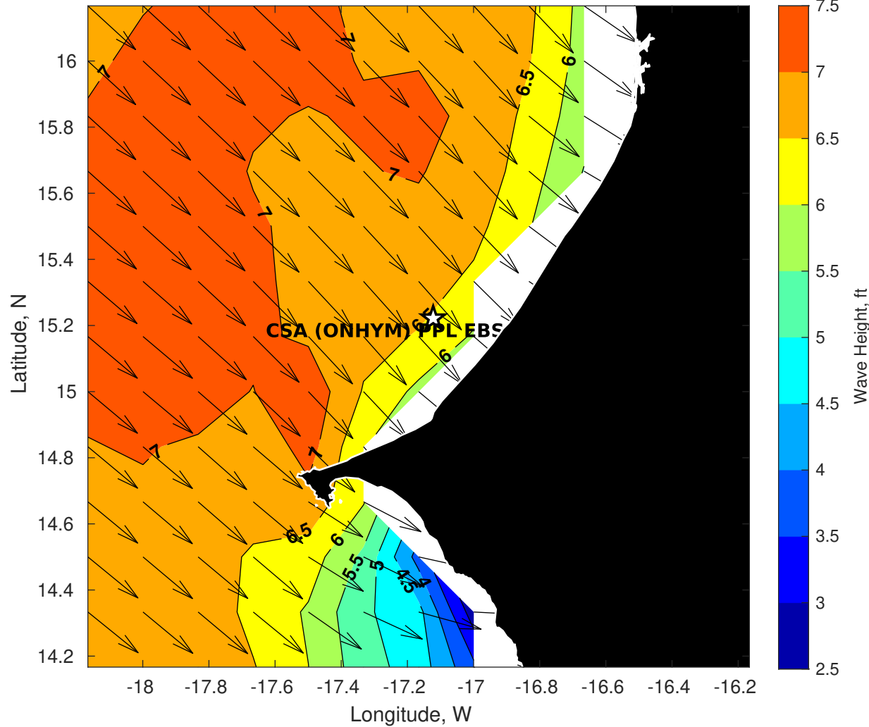
Wave Height (ft) for CSA (ONHYM) PPL EBS - Senegal at 12-Nov-2025 09:00:00
