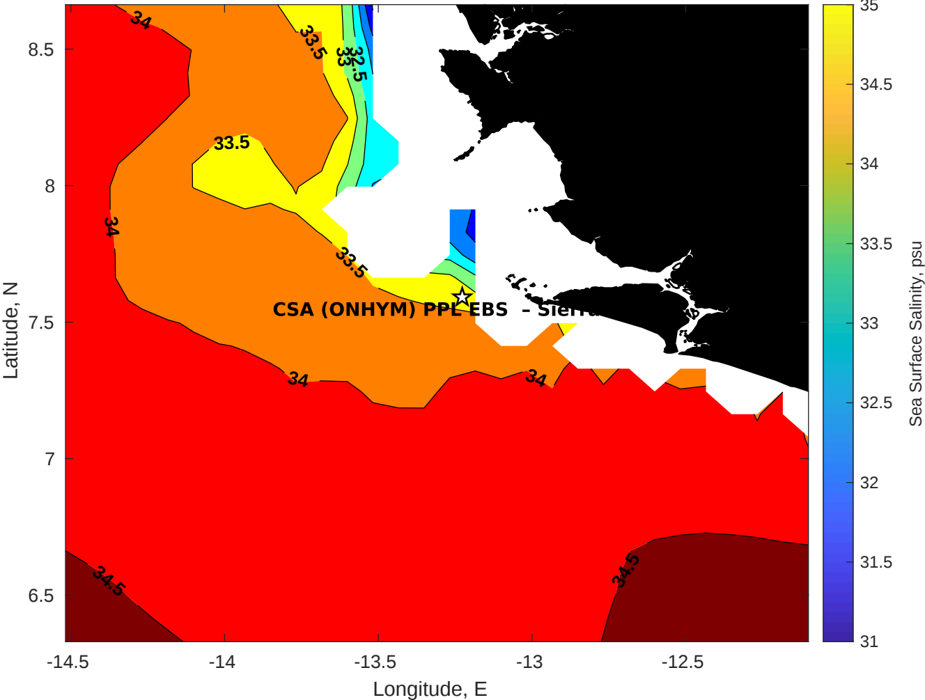
Surface Salinity for CSA (ONHYM) PPL EBS - Sierra Leone at 11-Nov-2025 00:00:00
