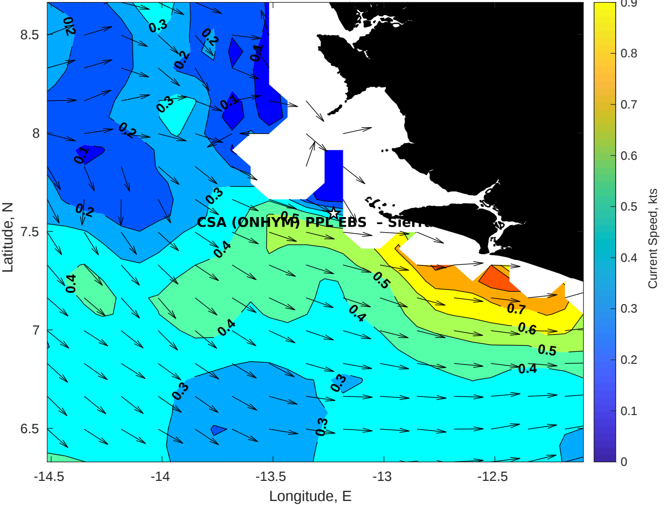
Surface Currents for CSA (ONHYM) PPL EBS - Sierra Leone at 11-Nov-2025 00:00:00
