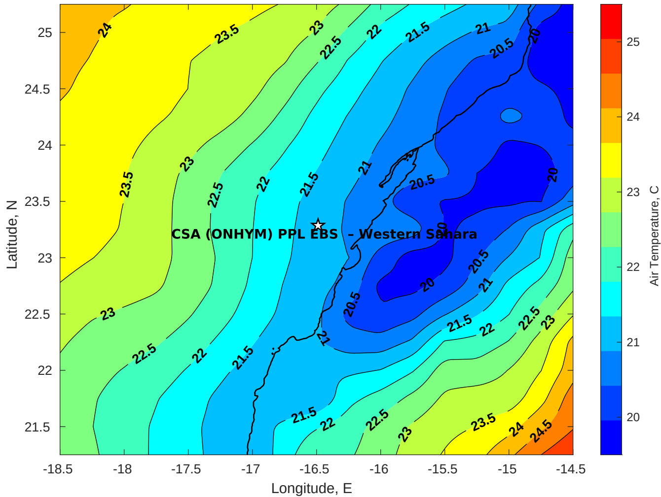
Air Temperature (C) for CSA (ONHYM) PPL EBS - Western Sahara at 12-Nov-2025
