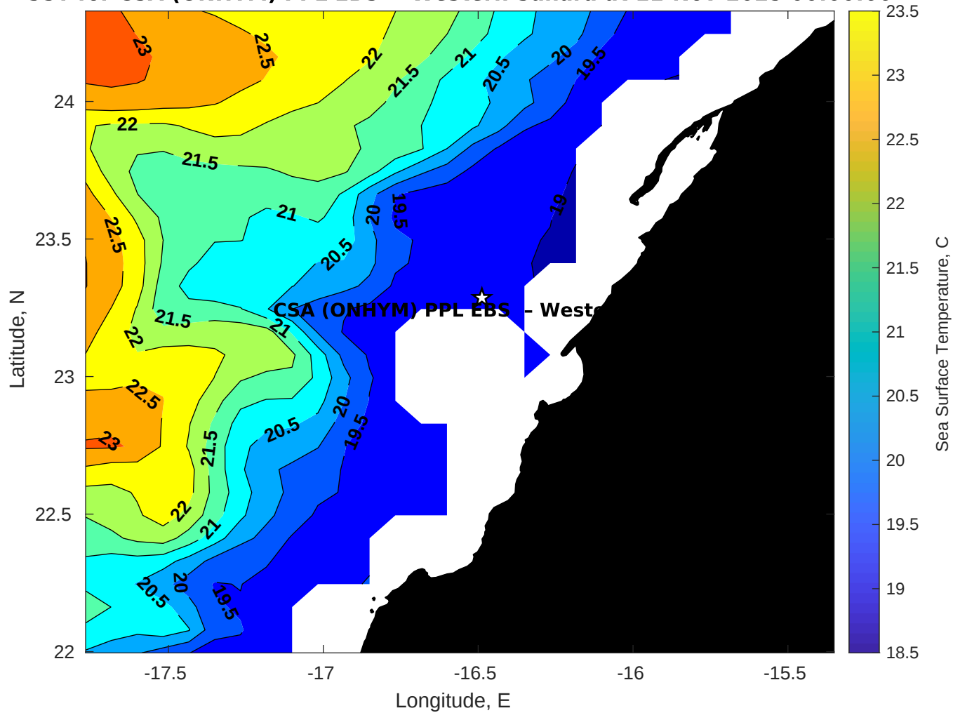
SST for CSA (ONHYM) PPL EBS - Western Sahara at 11-Nov-2025 00:00:00
