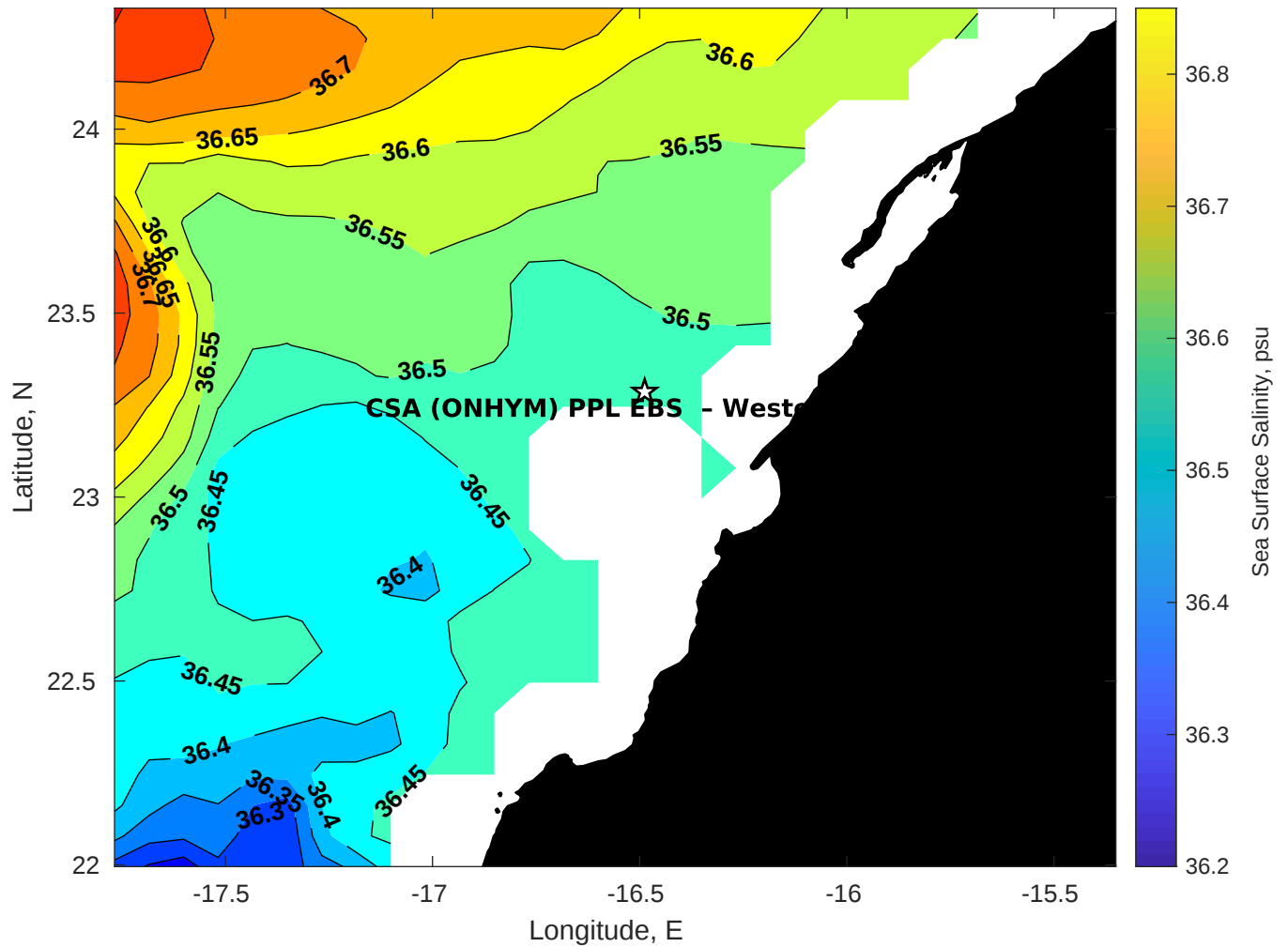
Surface Salinity for CSA (ONHYM) PPL EBS - Western Sahara at 11-Nov-2025 00:00:00
