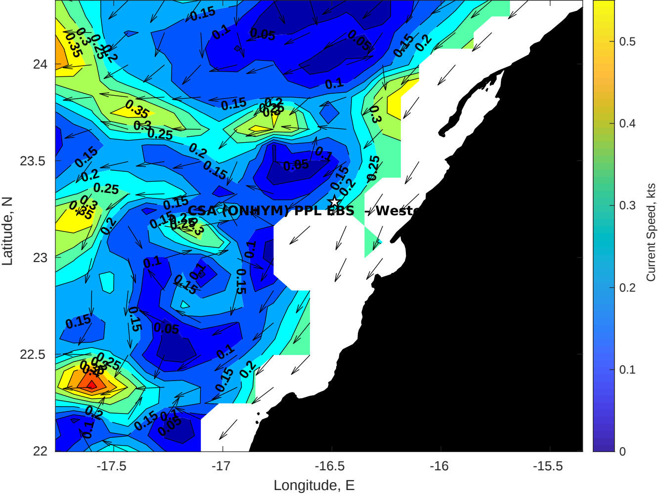
Surface Currents for CSA (ONHYM) PPL EBS - Western Sahara at 11-Nov-2025 00:00:00
