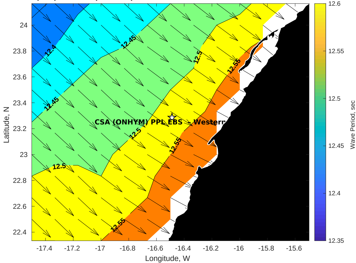
Wave Period (sec) for CSA (ONHYM) PPL EBS - Western Sahara at 12-Nov-2025 09:00:00
