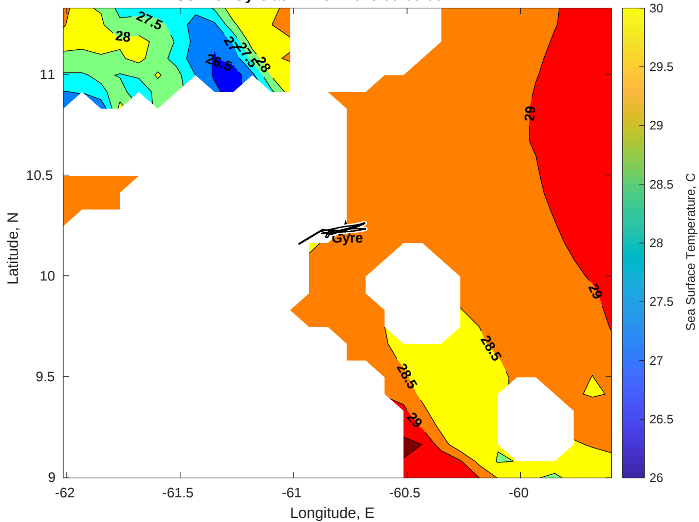
SST for Gyre at 11-Nov-2025 00:00:00
