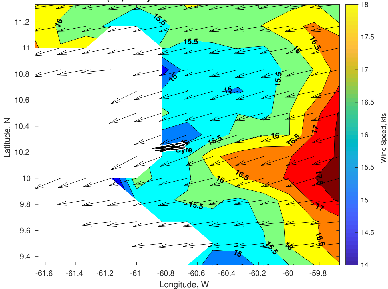
Winds (kts) for Gyre at 12-Nov-2025 09:00:00
