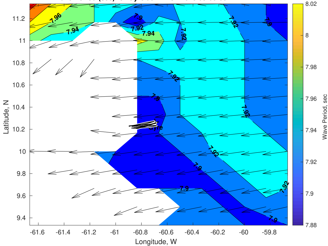
Wave Period (sec) for Gyre at 12-Nov-2025 09:00:00
