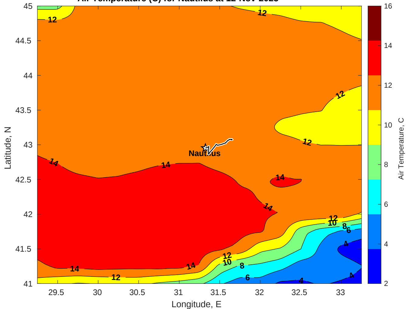
Air Temperature (C) for Nautilus at 12-Nov-2025
