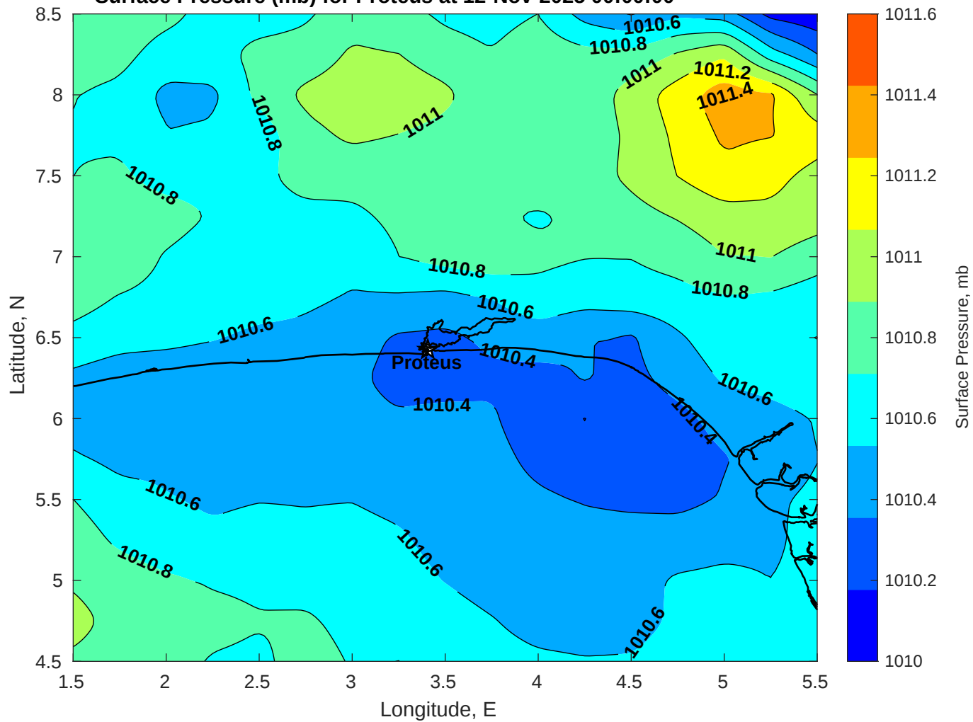
Surface Pressure (mb) for Proteus at 12-Nov-2025 00:00:00
