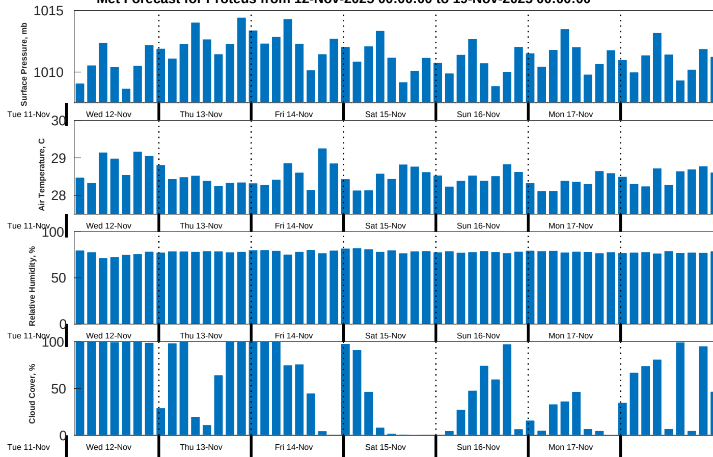
Met Forecast for Proteus from 12-Nov-2025 00:00:00 to 19-Nov-2025 00:00:00
