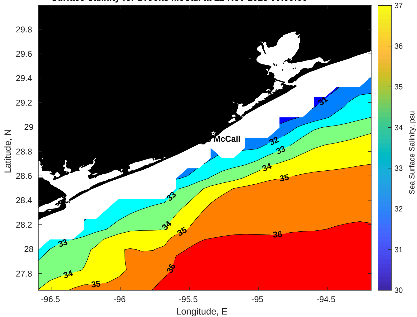
Surface Salinity for Brooks McCall at 12-Nov-2025 00:00:00
