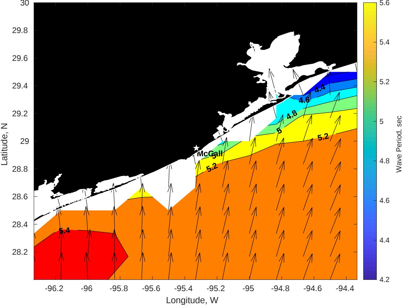
Wave Period (sec) for Brooks McCall at 13-Nov-2025 09:00:00
