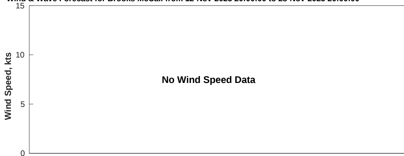
Wind & Wave Forecast for Brooks McCall from 12-Nov-2025 20:00:00 to 28-Nov-2025 20:00:00
