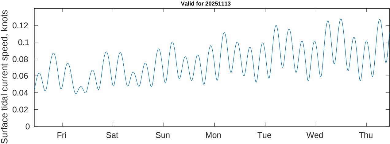
Tidal Currents and Heights for CSA (ONHYM) PPL EBS - Cote d'Ivoire at 20251113
