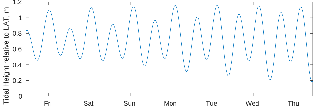
Tidal Currents and Heights for CSA (ONHYM) PPL EBS - Cote d'Ivoire at 20251113
