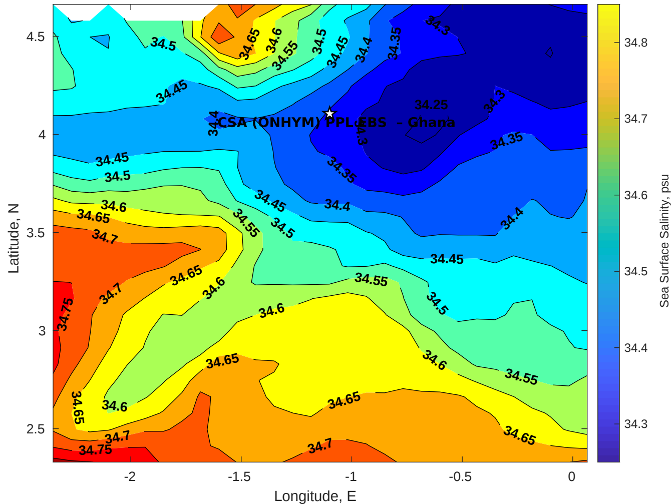
Surface Salinity for CSA (ONHYM) PPL EBS - Ghana at 12-Nov-2025 00:00:00
