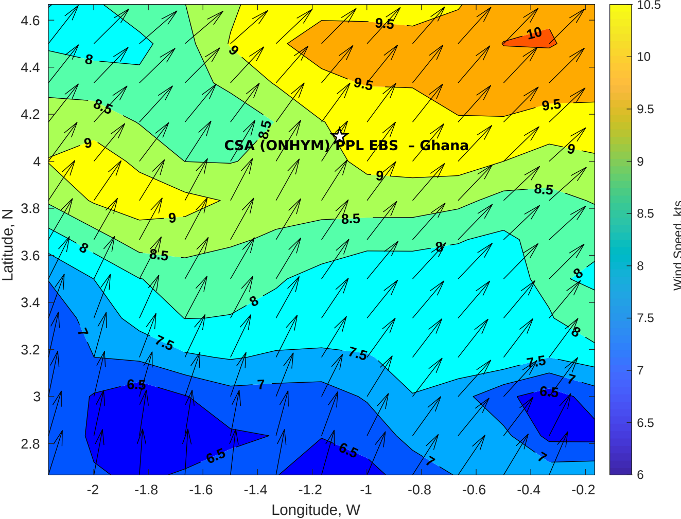
Winds (kts) for CSA (ONHYM) PPL EBS - Ghana at 13-Nov-2025 09:00:00
