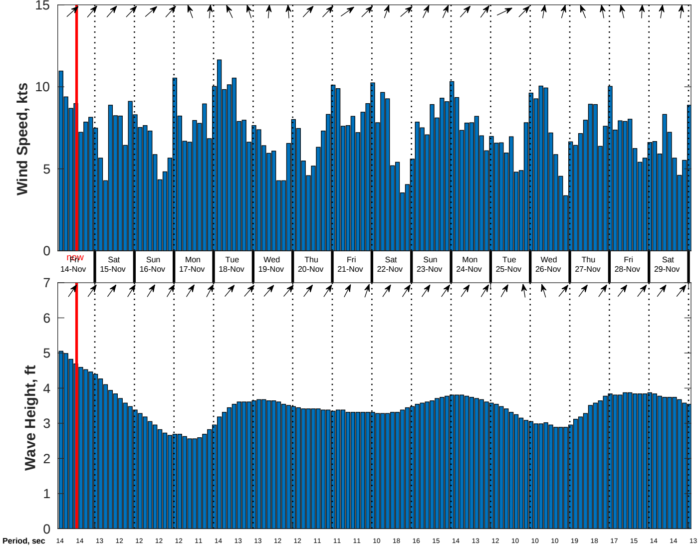
Wind & Wave Forecast for CSA (ONHYM) PPL EBS - Ghana from 13-Nov-2025 02:00:00 to 29-Nov-2025 02:00:00
