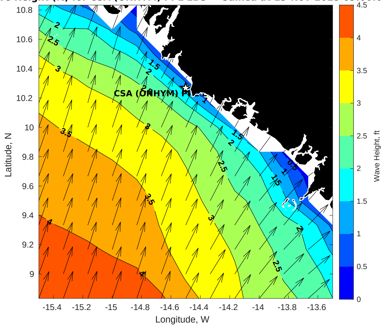
Wave Height (ft) for CSA (ONHYM) PPL EBS - Guinea at 13-Nov-2025 09:00:00
