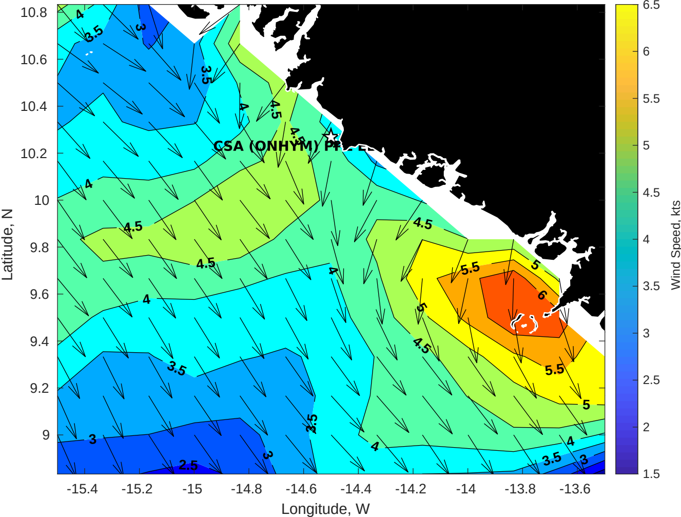
Winds (kts) for CSA (ONHYM) PPL EBS - Guinea at 13-Nov-2025 09:00:00
