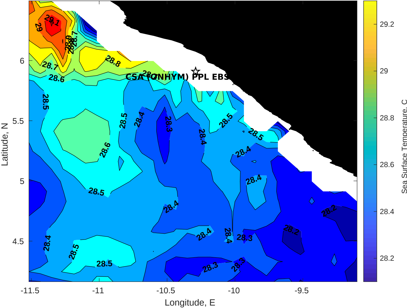
SST for CSA (ONHYM) PPL EBS - Liberia at 12-Nov-2025 00:00:00
