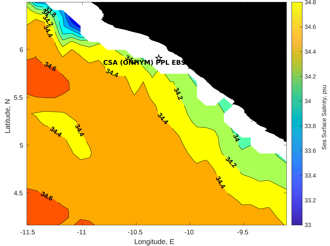
Surface Salinity for CSA (ONHYM) PPL EBS - Liberia at 12-Nov-2025 00:00:00
