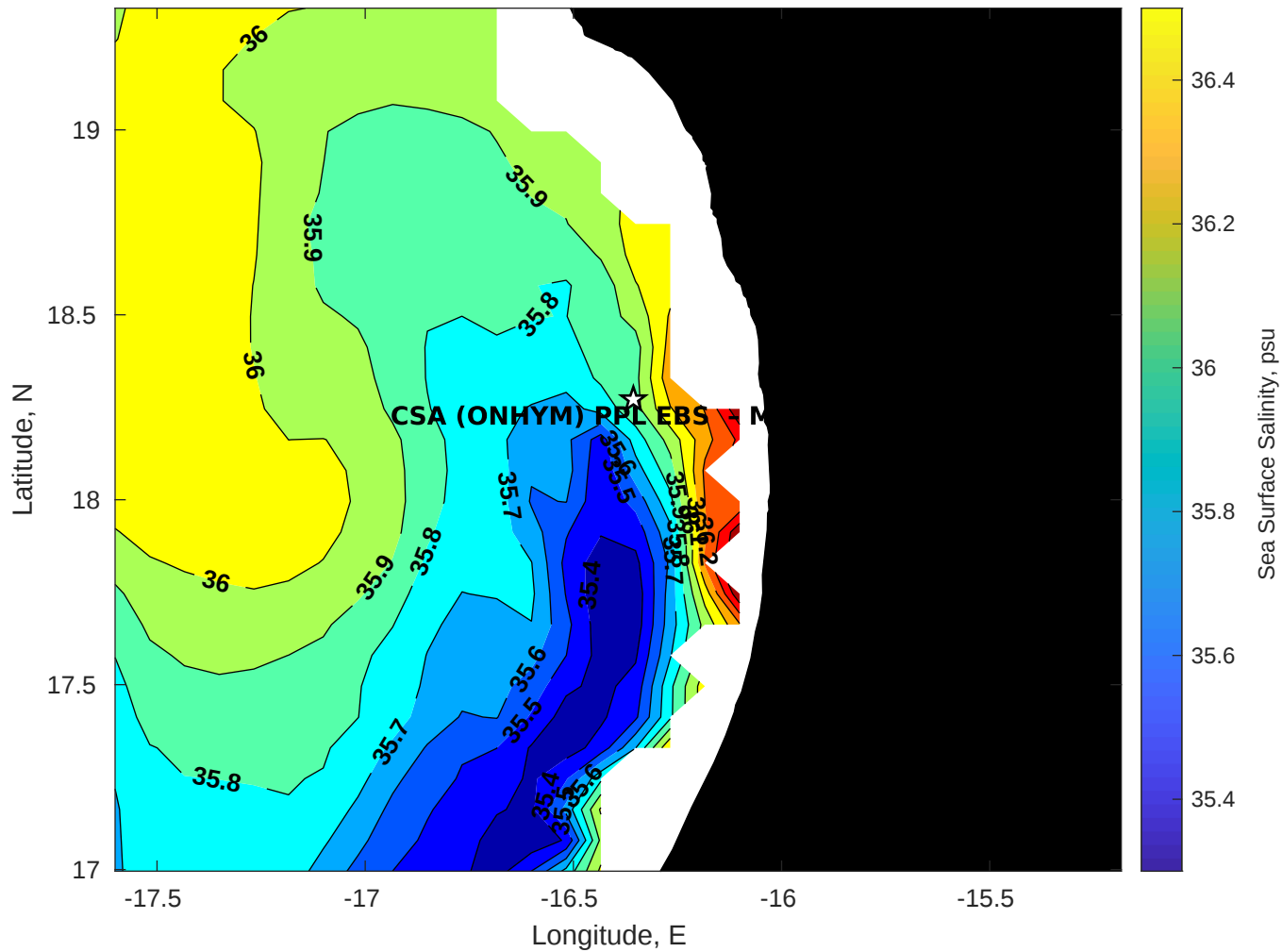
Surface Salinity for CSA (ONHYM) PPL EBS - Mauritania at 12-Nov-2025 00:00:00
