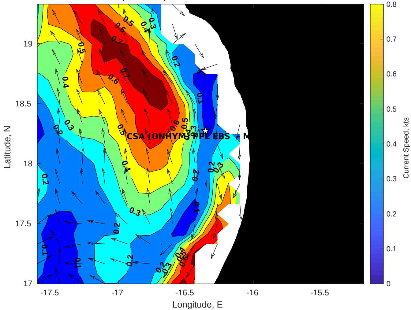
Surface Currents for CSA (ONHYM) PPL EBS - Mauritania at 12-Nov-2025 00:00:00
