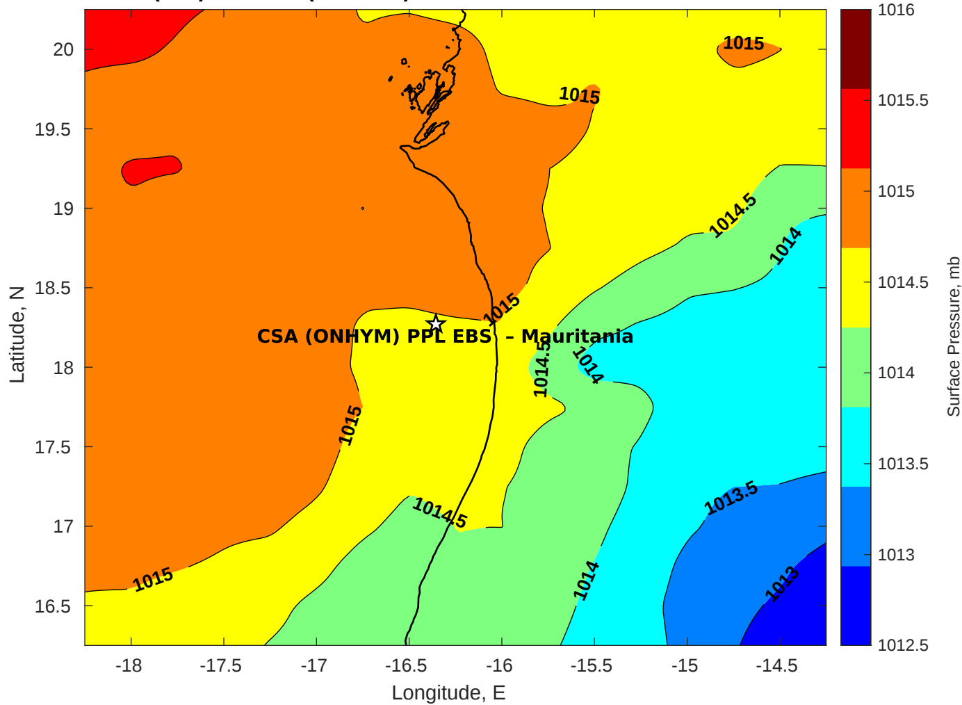
Surface Pressure (mb) for CSA (ONHYM) PPL EBS - Mauritania at 13-Nov-2025 00:00:00
