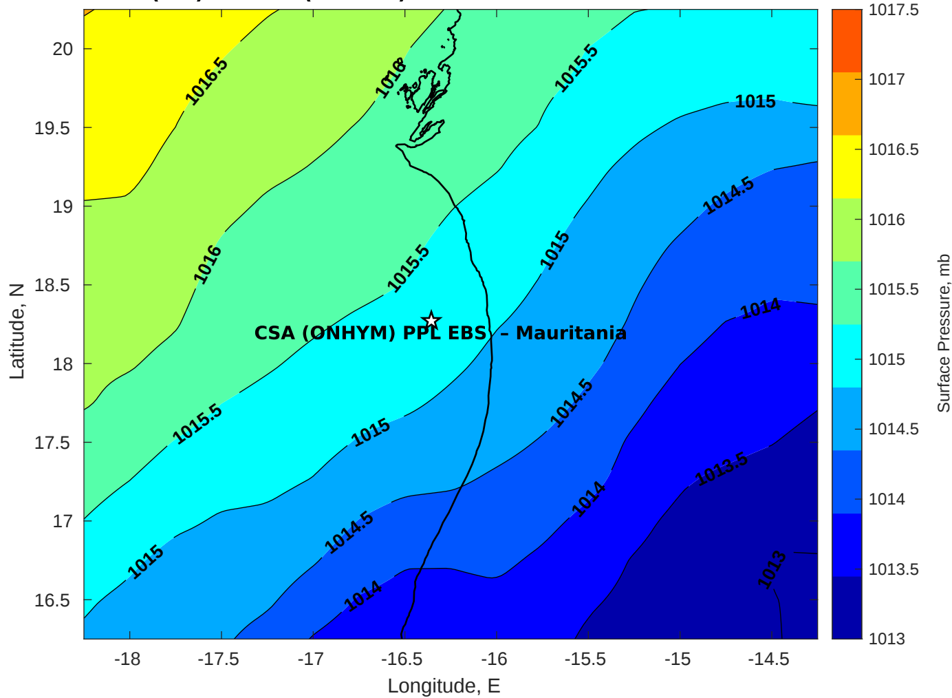
Surface Pressure (mb) for CSA (ONHYM) PPL EBS - Mauritania at 15-Nov-2025 00:00:00
