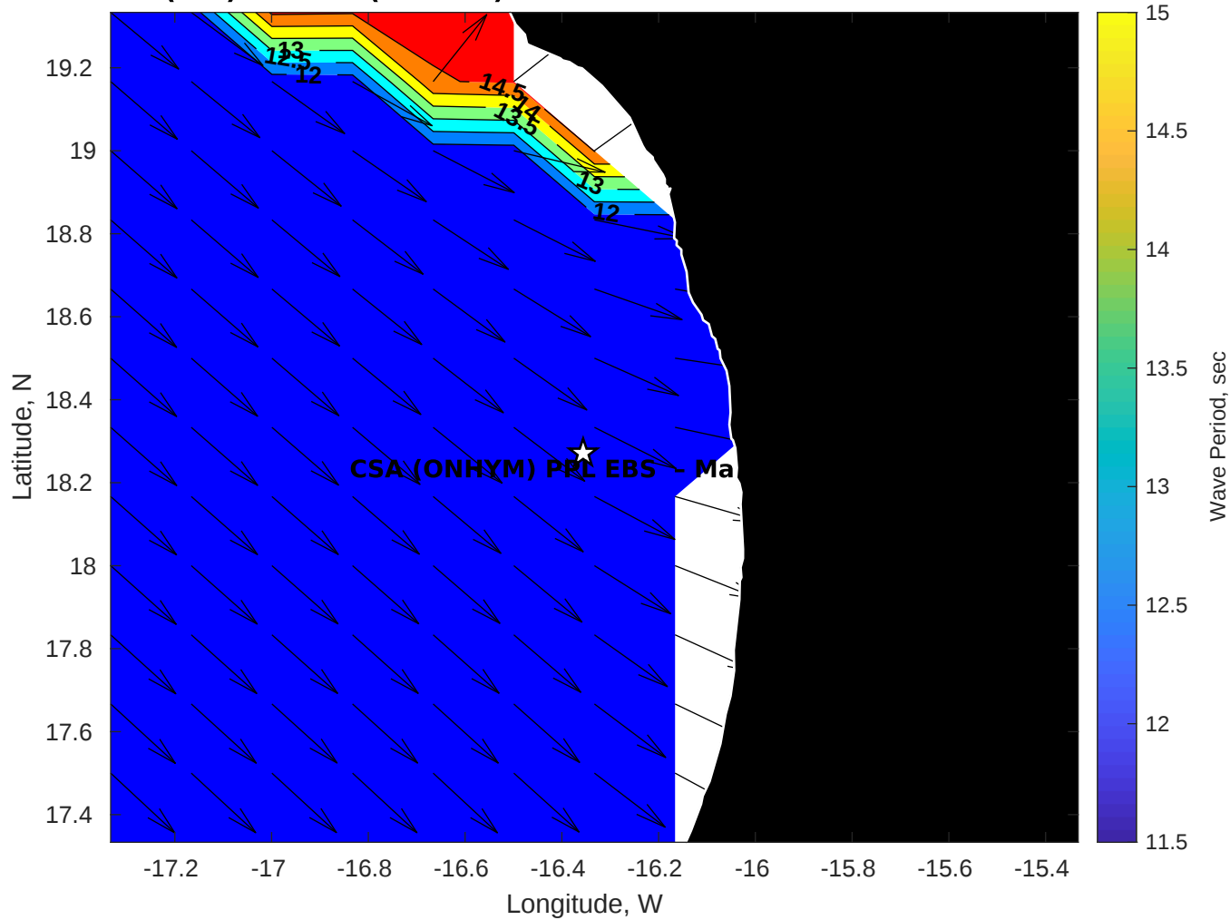
Wave Period (sec) for CSA (ONHYM) PPL EBS - Mauritania at 13-Nov-2025 09:00:00
