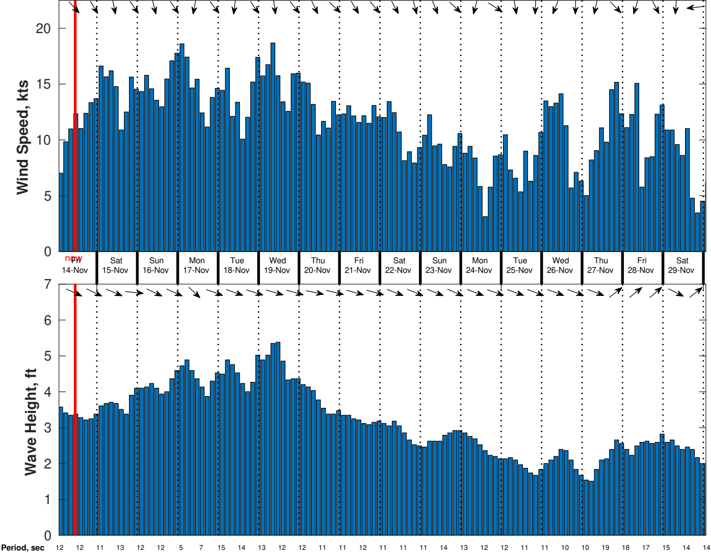
Wind & Wave Forecast for CSA (ONHYM) PPL EBS - Mauritania from 13-Nov-2025 01:00:00 to 29-Nov-2025 01:00:00
