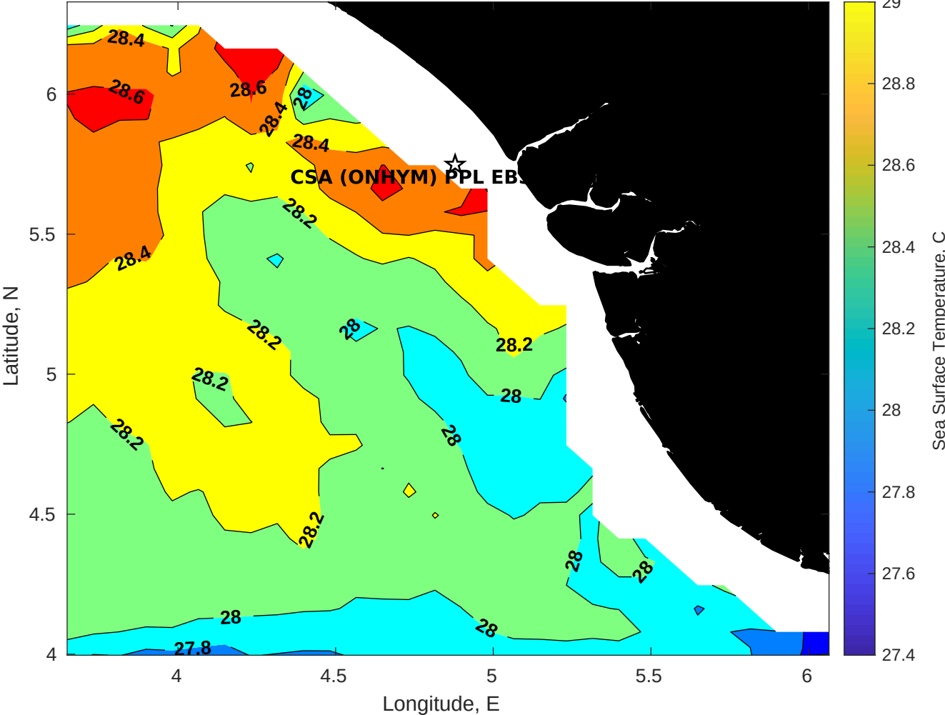
SST for CSA (ONHYM) PPL EBS - Nigeria at 12-Nov-2025 00:00:00
