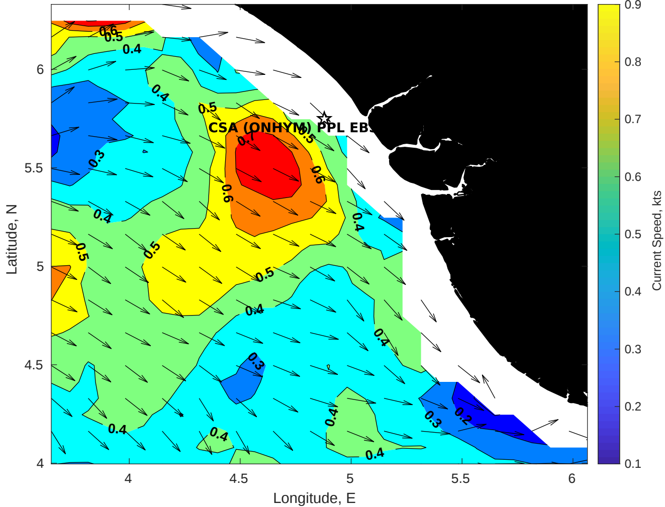
Surface Currents for CSA (ONHYM) PPL EBS - Nigeria at 12-Nov-2025 00:00:00
