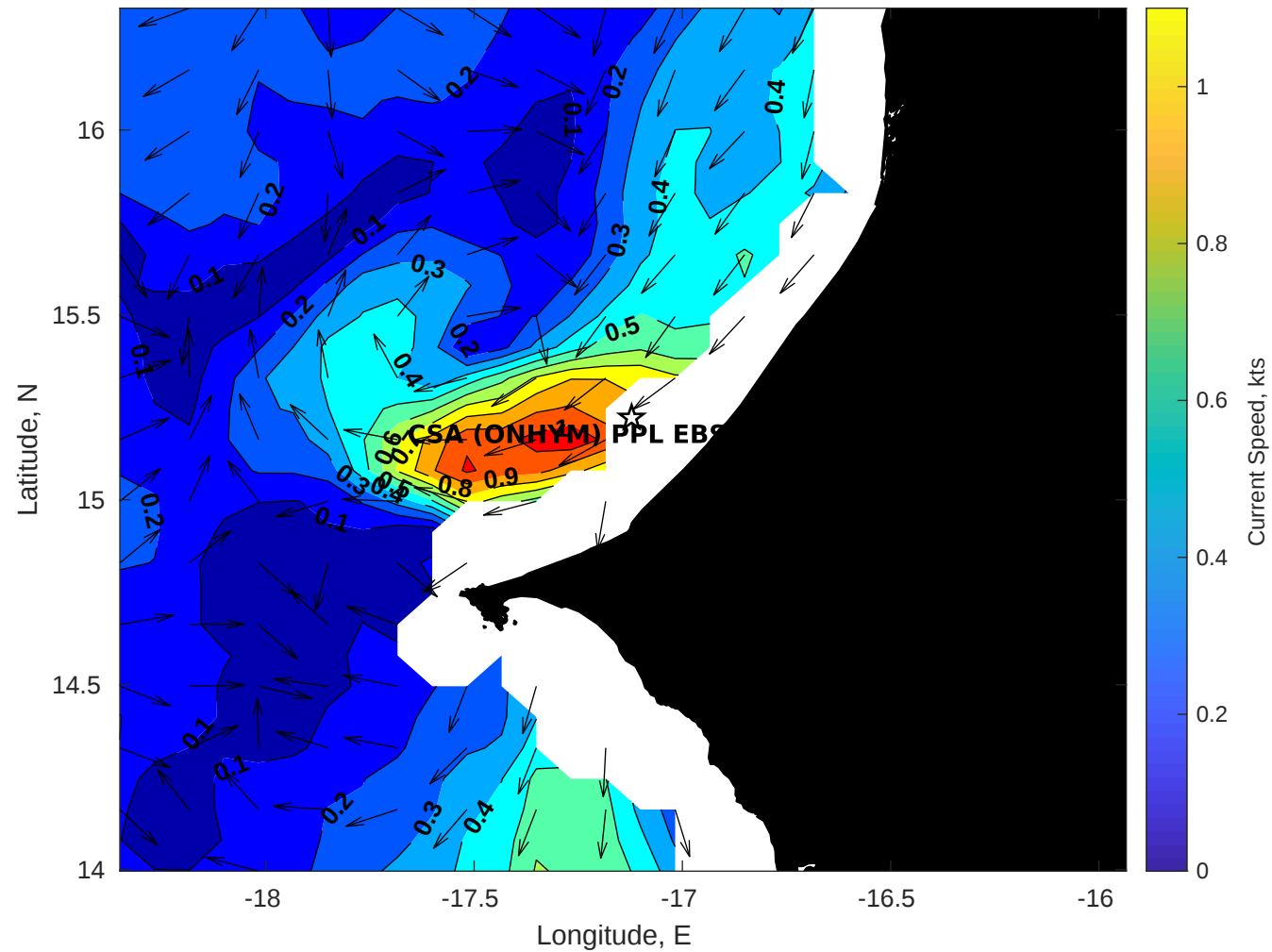
Surface Currents for CSA (ONHYM) PPL EBS - Senegal at 12-Nov-2025 00:00:00
