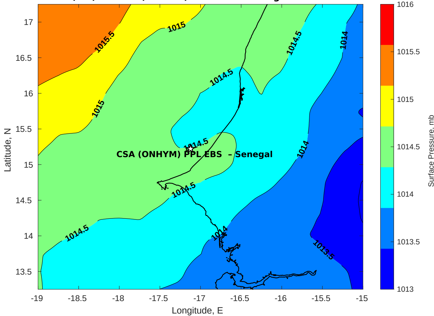
Surface Pressure (mb) for CSA (ONHYM) PPL EBS - Senegal at 14-Nov-2025 00:00:00
