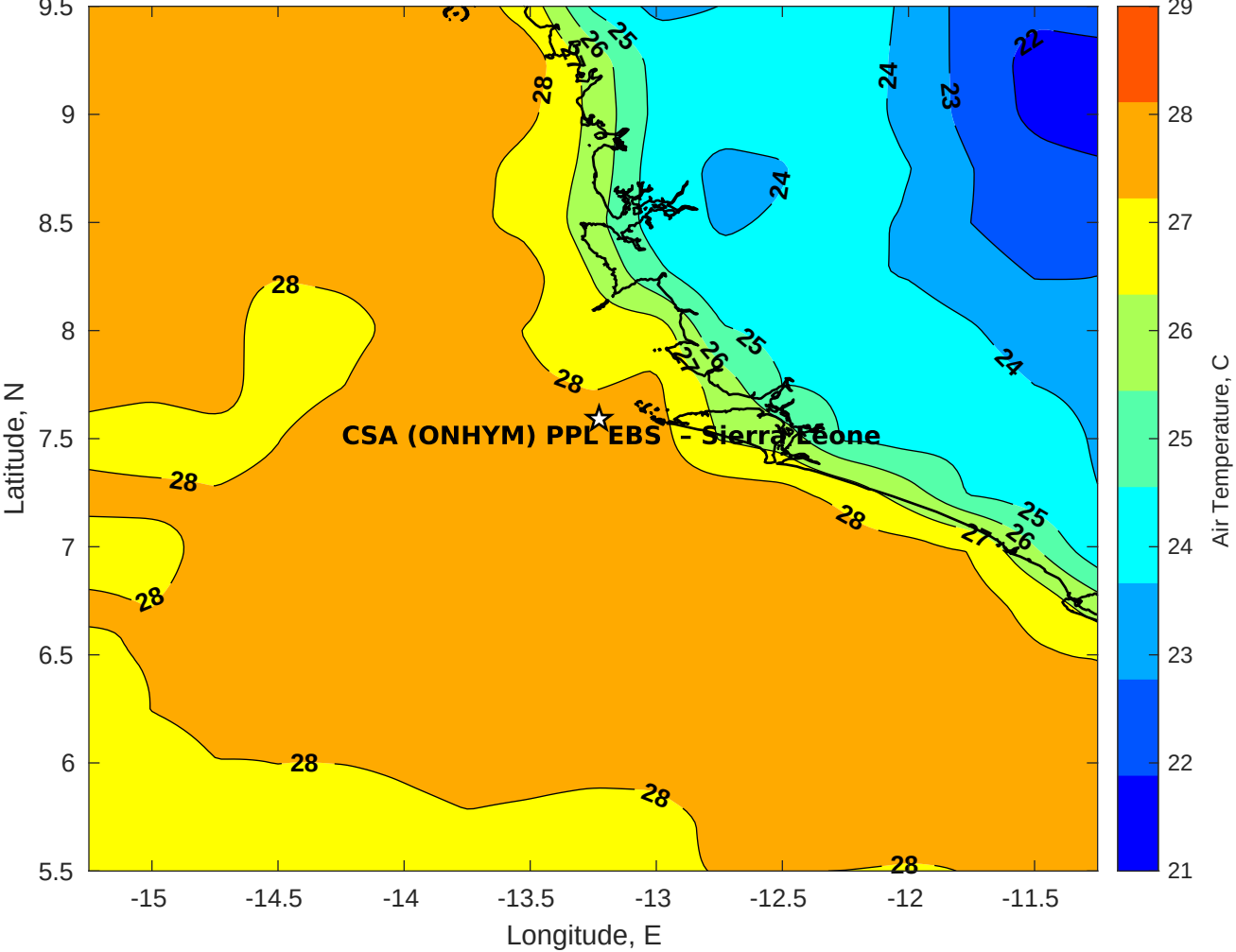
Air Temperature (C) for CSA (ONHYM) PPL EBS - Sierra Leone at 13-Nov-2025
