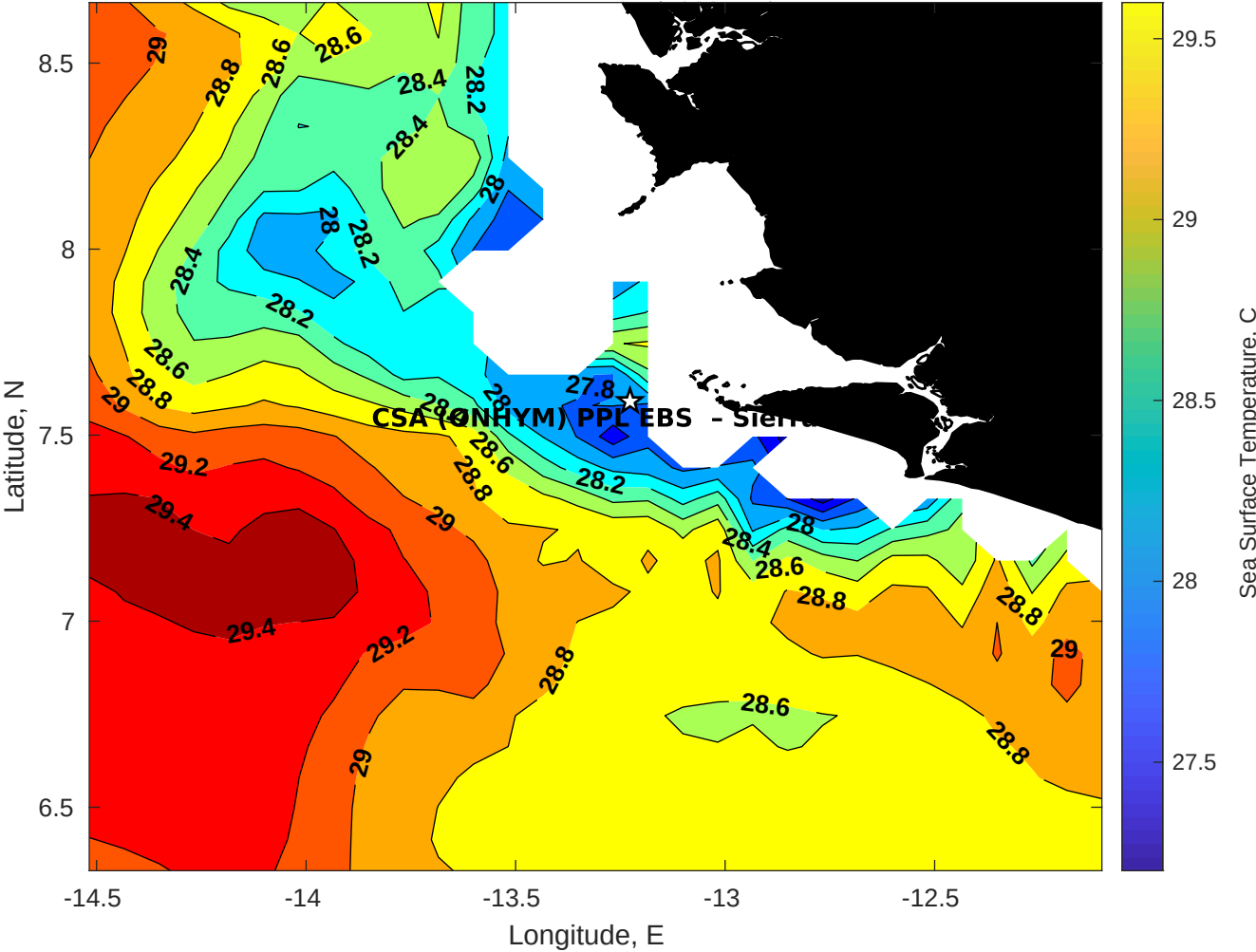
SST for CSA (ONHYM) PPL EBS - Sierra Leone at 12-Nov-2025 00:00:00
