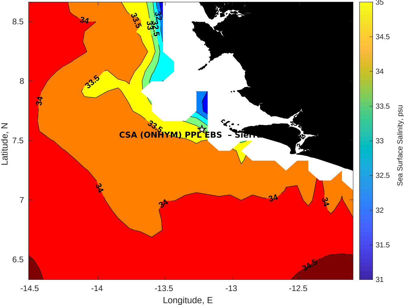
Surface Salinity for CSA (ONHYM) PPL EBS - Sierra Leone at 12-Nov-2025 00:00:00
