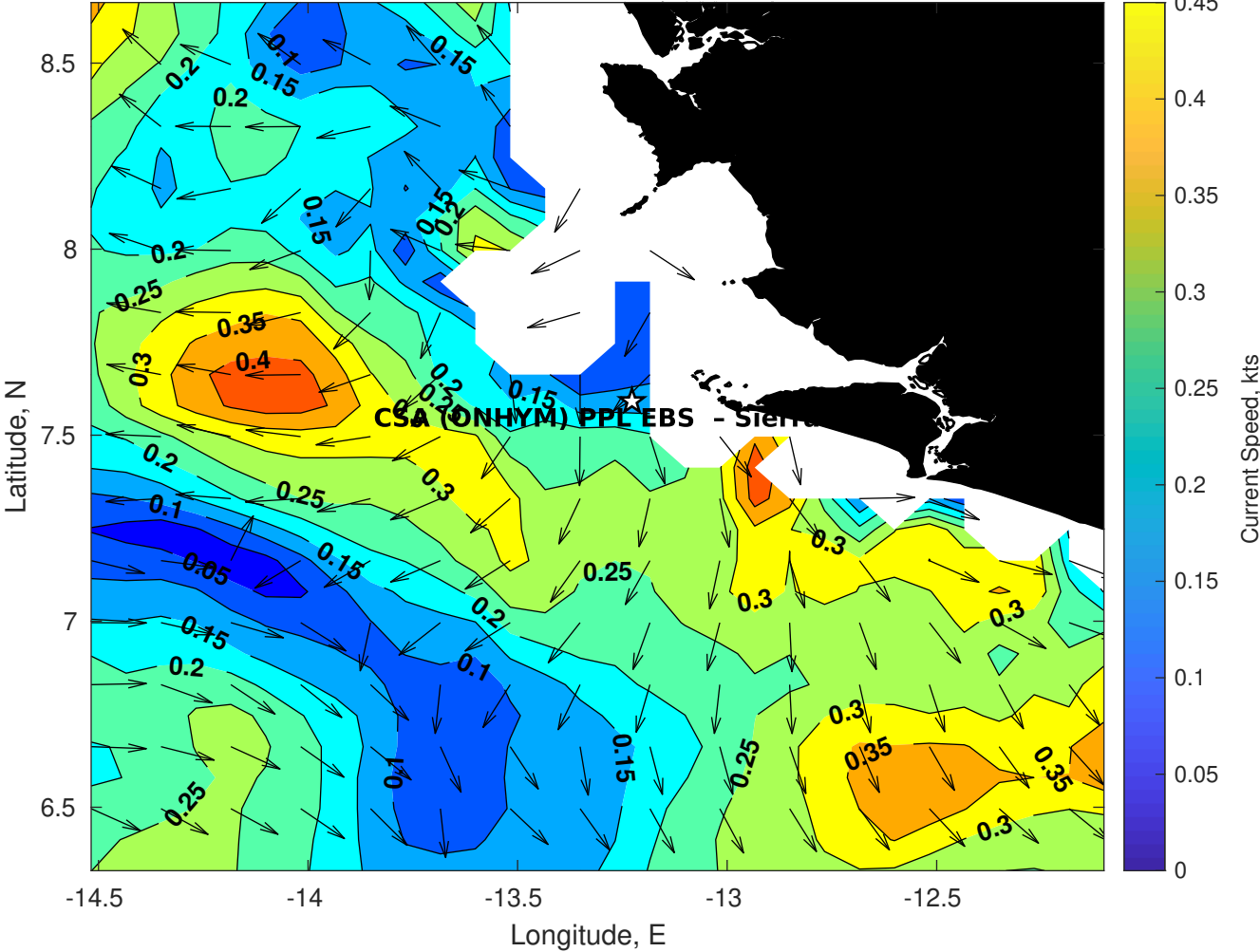
Surface Currents for CSA (ONHYM) PPL EBS - Sierra Leone at 12-Nov-2025 00:00:00
