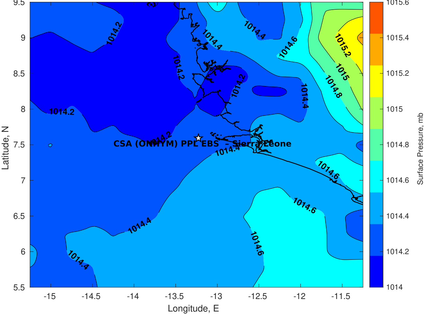
Surface Pressure (mb) for CSA (ONHYM) PPL EBS - Sierra Leone at 14-Nov-2025 00:00:00
