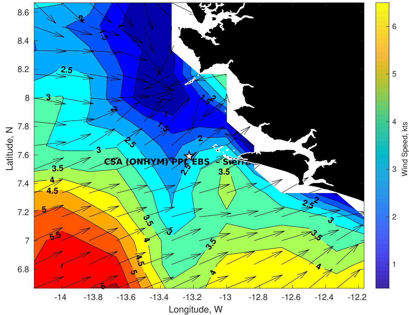
Winds (kts) for CSA (ONHYM) PPL EBS - Sierra Leone at 13-Nov-2025 09:00:00
