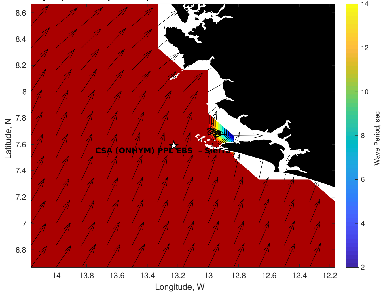
Wave Period (sec) for CSA (ONHYM) PPL EBS - Sierra Leone at 13-Nov-2025 09:00:00
