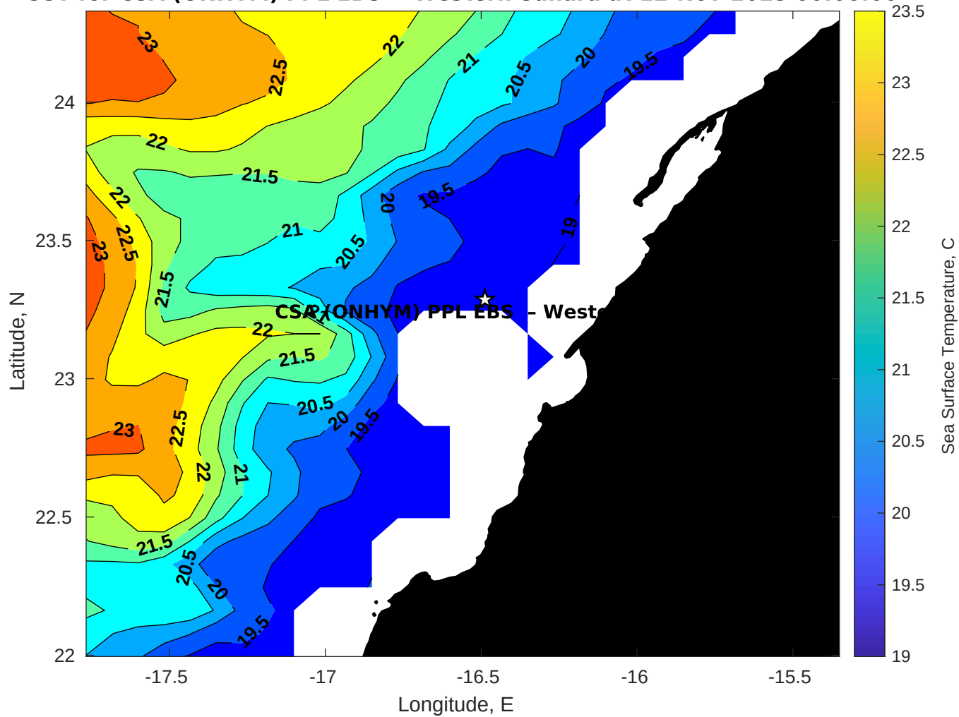
SST for CSA (ONHYM) PPL EBS - Western Sahara at 12-Nov-2025 00:00:00
