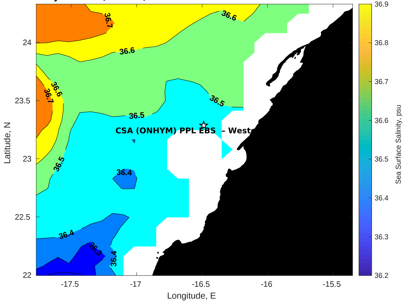
Surface Salinity for CSA (ONHYM) PPL EBS - Western Sahara at 12-Nov-2025 00:00:00
