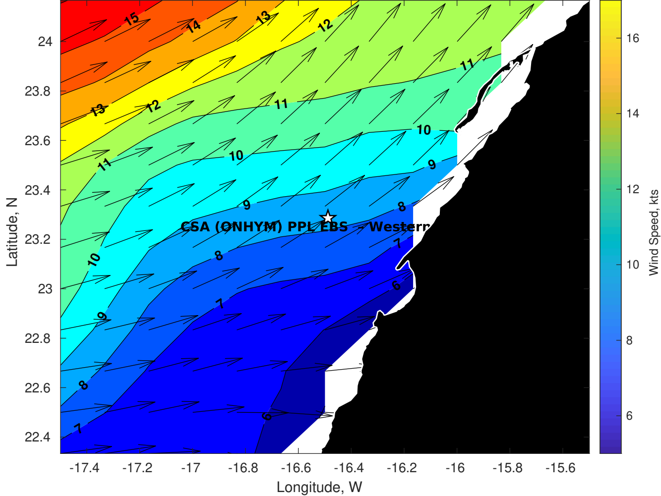
Winds (kts) for CSA (ONHYM) PPL EBS - Western Sahara at 13-Nov-2025 09:00:00
