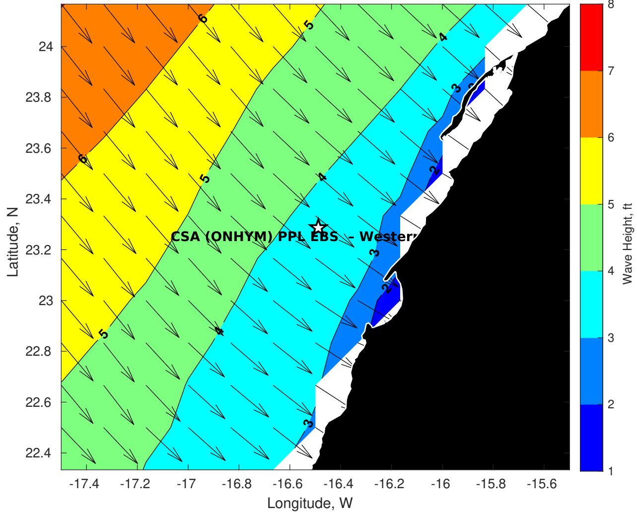
Wave Height (ft) for CSA (ONHYM) PPL EBS - Western Sahara at 13-Nov-2025 09:00:00
