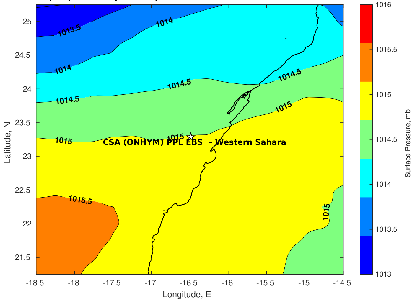
Surface Pressure (mb) for CSA (ONHYM) PPL EBS - Western Sahara at 13-Nov-2025 00:00:00
