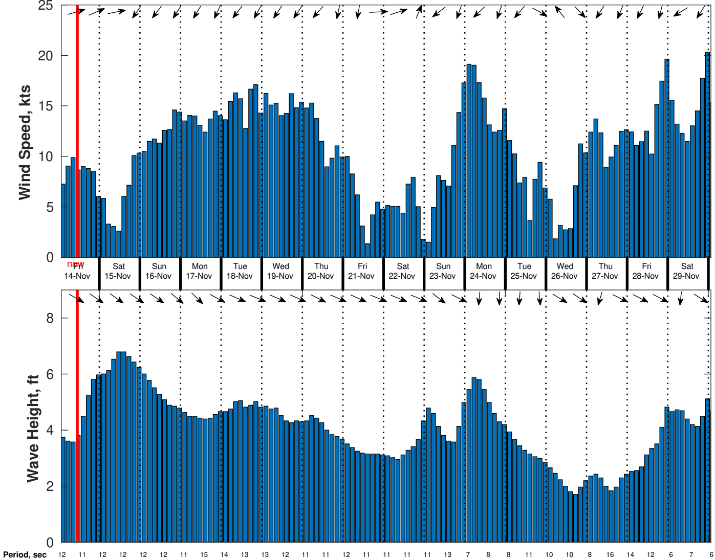
Wind & Wave Forecast for CSA (ONHYM) PPL EBS - Western Sahara from 13-Nov-2025 01:00:00 to 29-Nov-2025 01:00:00
