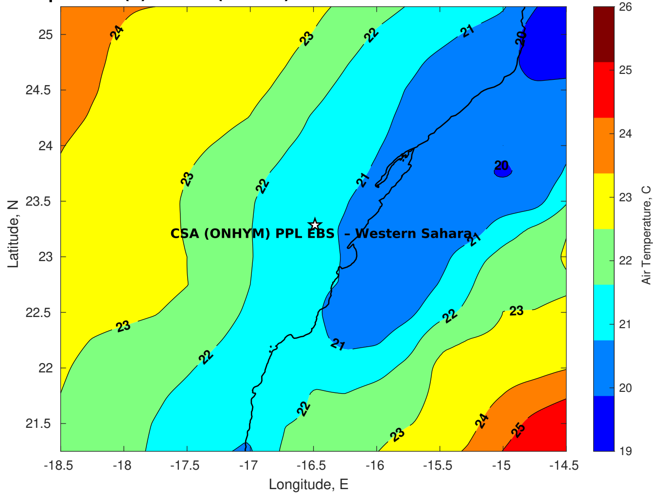
Air Temperature (C) for CSA (ONHYM) PPL EBS - Western Sahara at 13-Nov-2025
