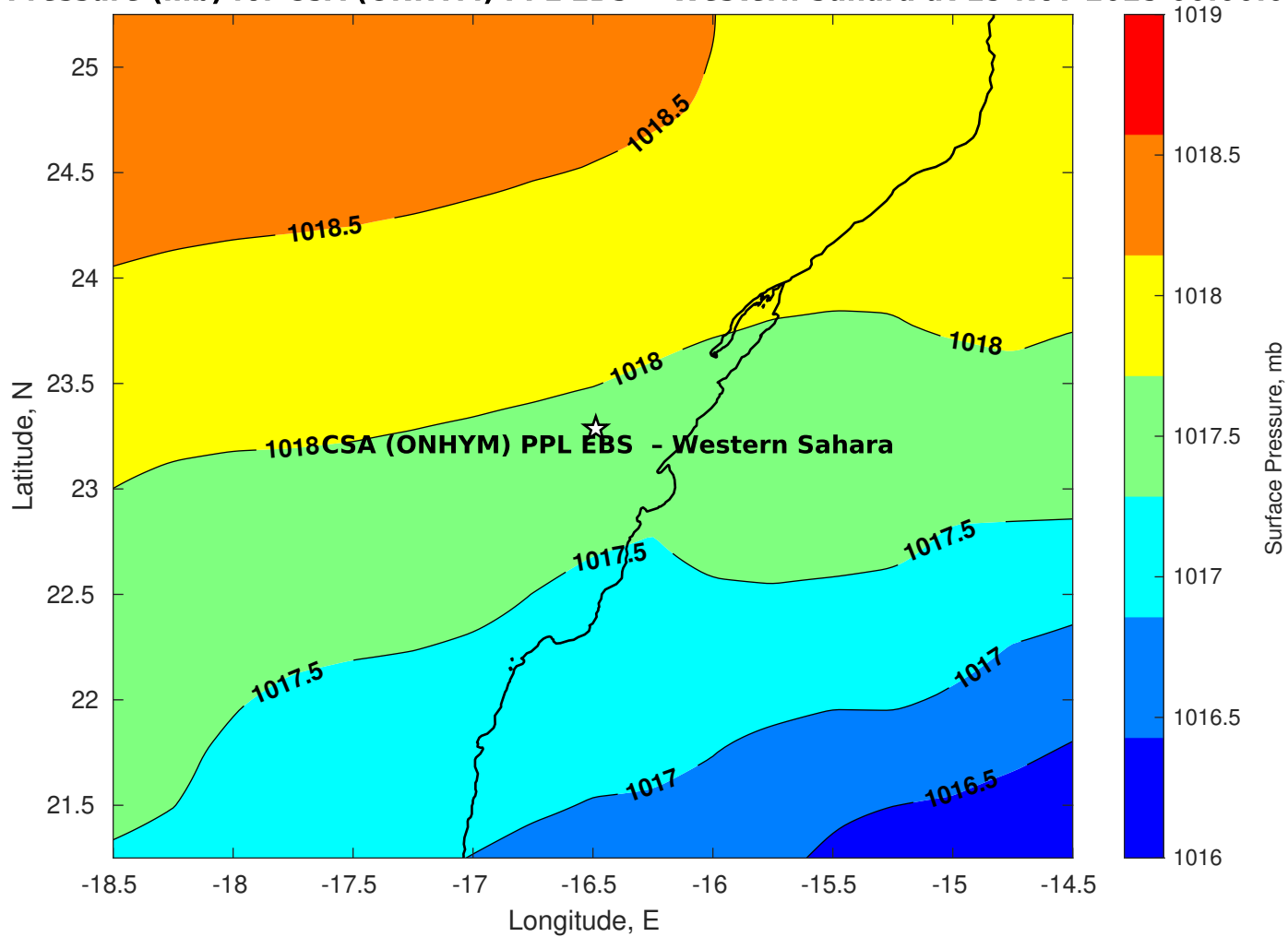
Surface Pressure (mb) for CSA (ONHYM) PPL EBS - Western Sahara at 15-Nov-2025 00:00:00
