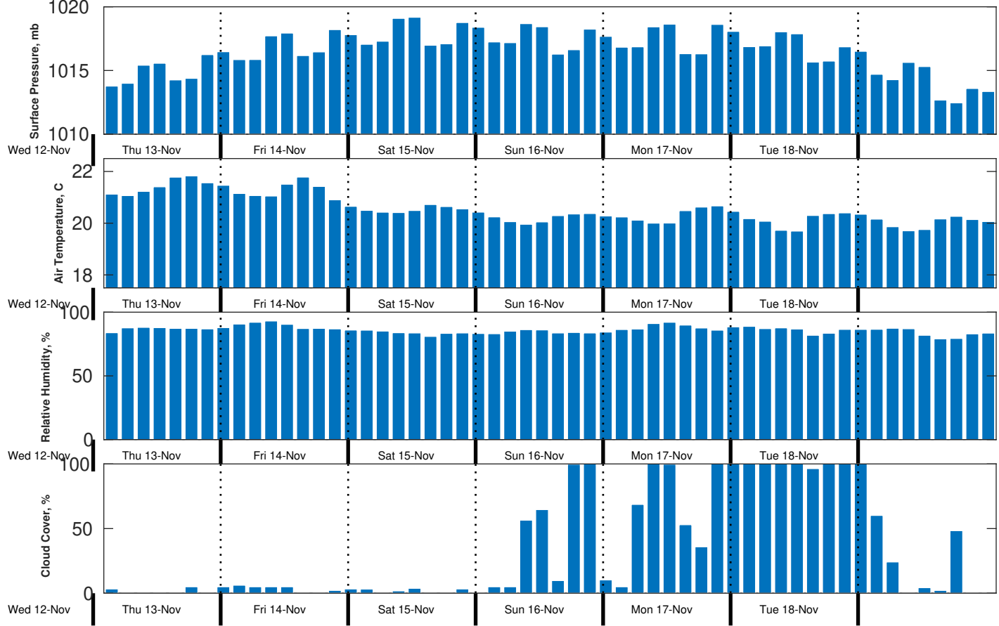
Met Forecast for CSA (ONHYM) PPL EBS - Western Sahara from 13-Nov-2025 00:00:00 to 20-Nov-2025 00:00:00
