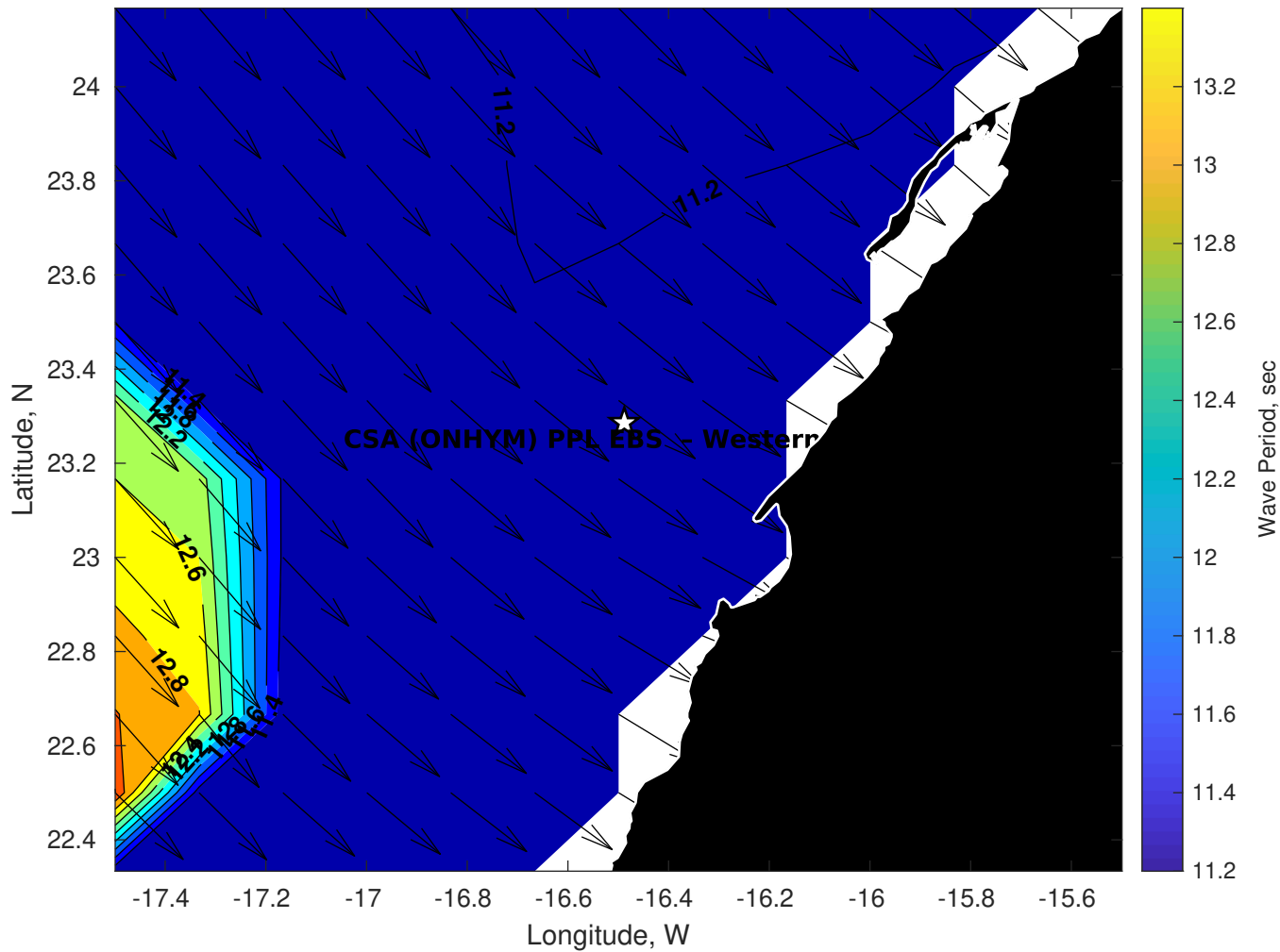
Wave Period (sec) for CSA (ONHYM) PPL EBS - Western Sahara at 13-Nov-2025 09:00:00
