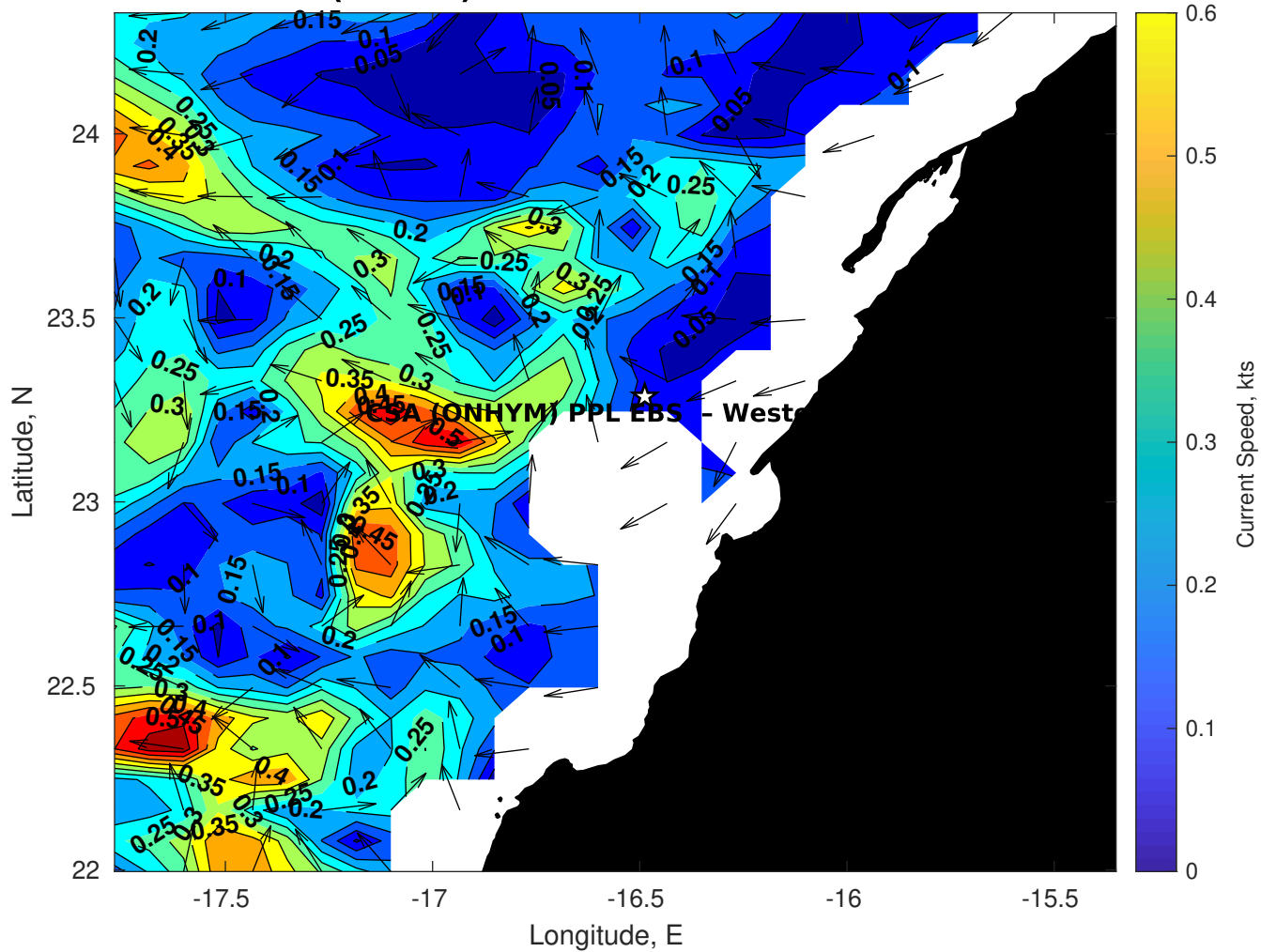
Surface Currents for CSA (ONHYM) PPL EBS - Western Sahara at 12-Nov-2025 00:00:00
