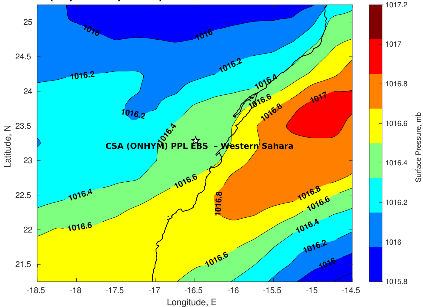
Surface Pressure (mb) for CSA (ONHYM) PPL EBS - Western Sahara at 14-Nov-2025 00:00:00
