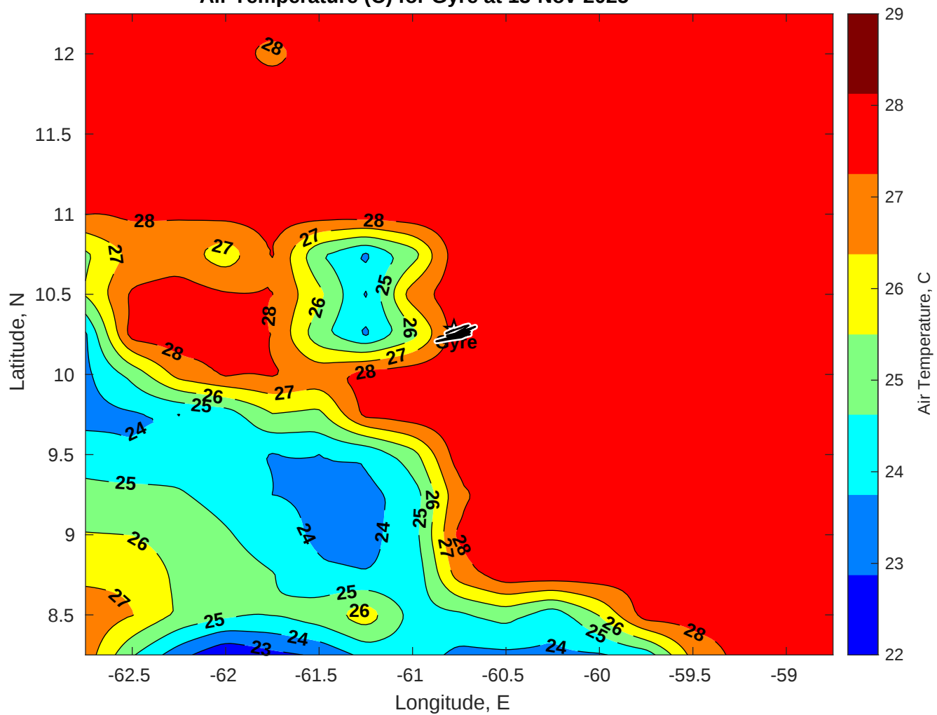
Air Temperature (C) for Gyre at 13-Nov-2025
