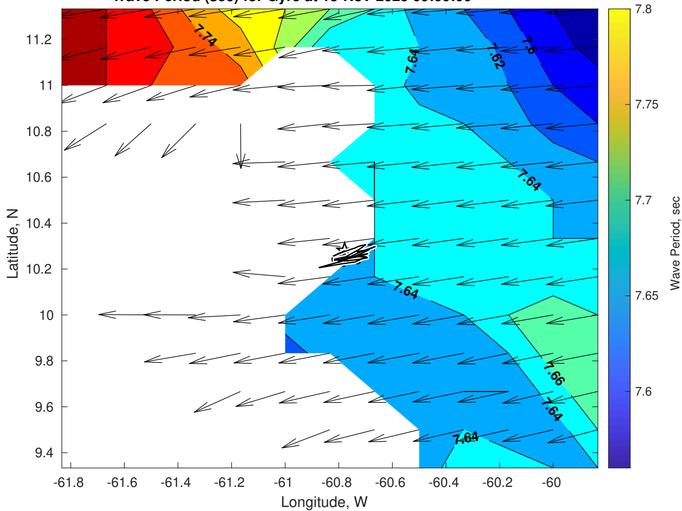
Wave Period (sec) for Gyre at 13-Nov-2025 09:00:00
