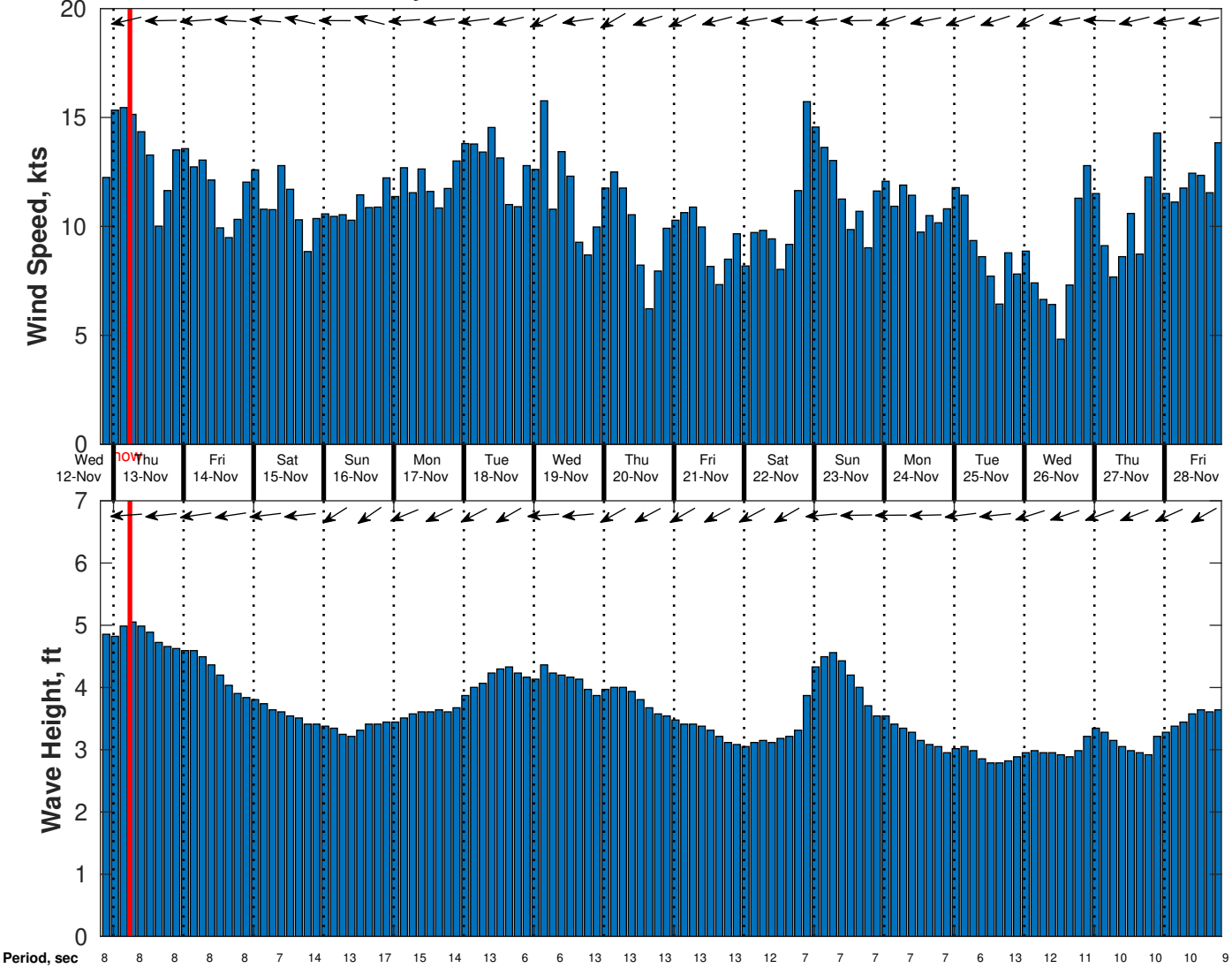
Wind & Wave Forecast for Gyre from 12-Nov-2025 20:00:00 to 28-Nov-2025 20:00:00
