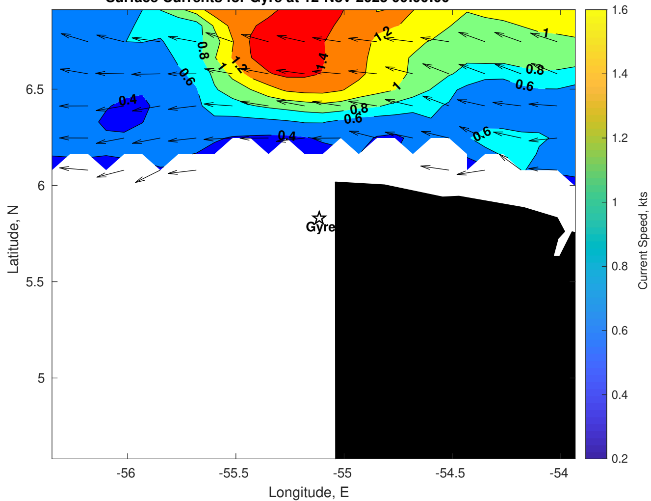
Surface Currents for Gyre at 12-Nov-2025 00:00:00
