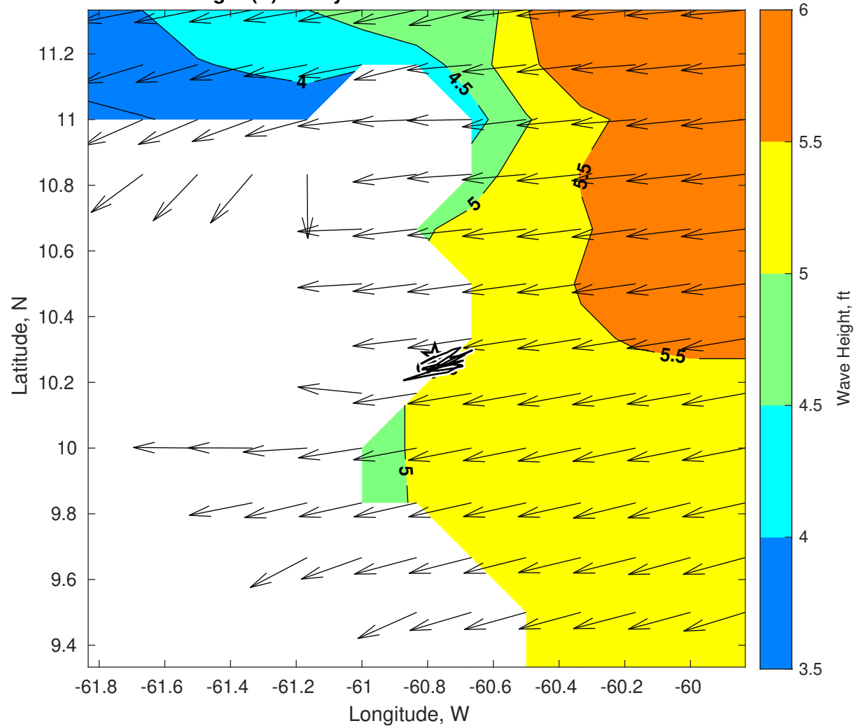
Wave Height (ft) for Gyre at 13-Nov-2025 09:00:00
