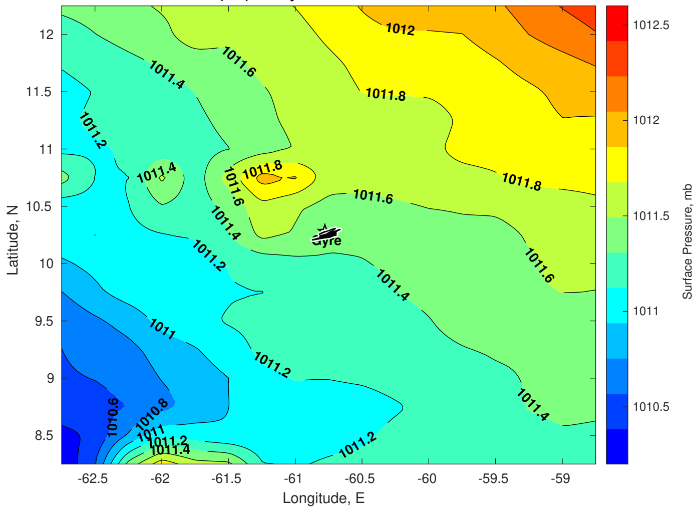
Surface Pressure (mb) for Gyre at 15-Nov-2025 00:00:00
