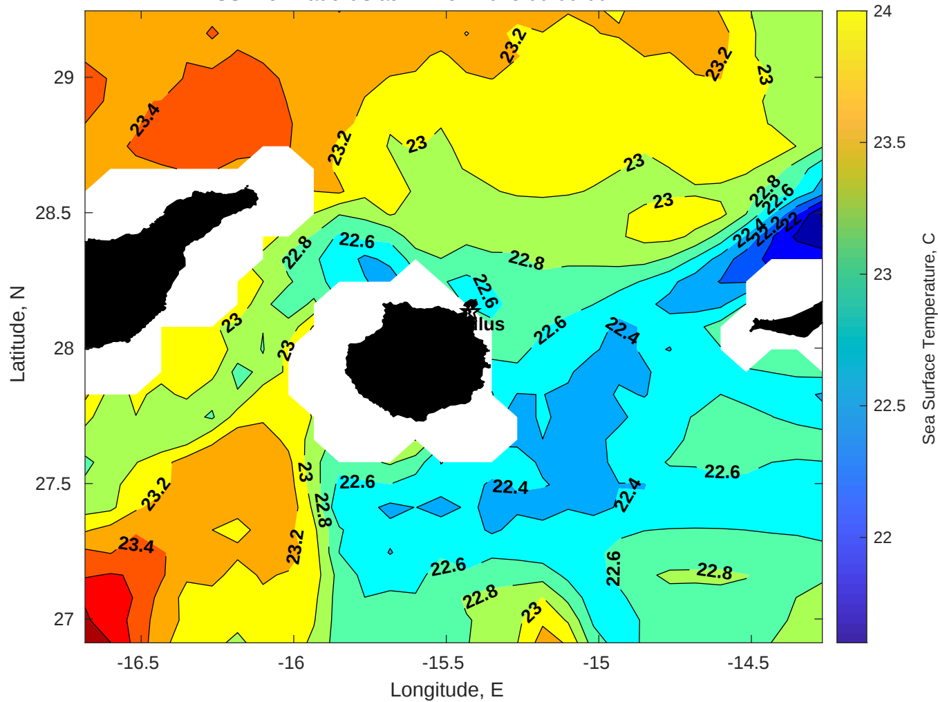
SST for Nautilus at 12-Nov-2025 00:00:00
