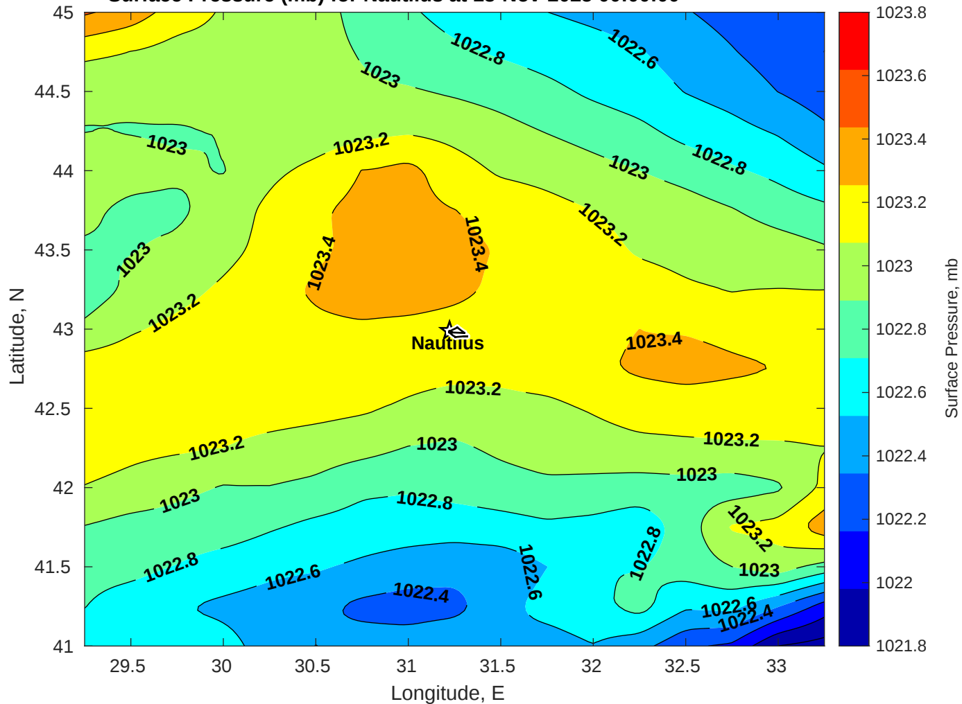
Surface Pressure (mb) for Nautilus at 13-Nov-2025 00:00:00
