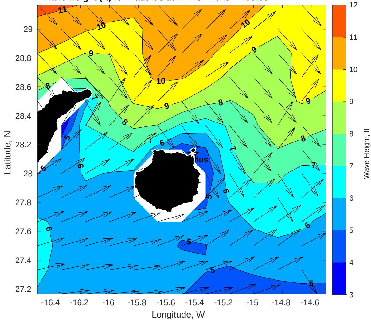
Wave Height (ft) for Nautilus at 12-Nov-2025 21:00:00
