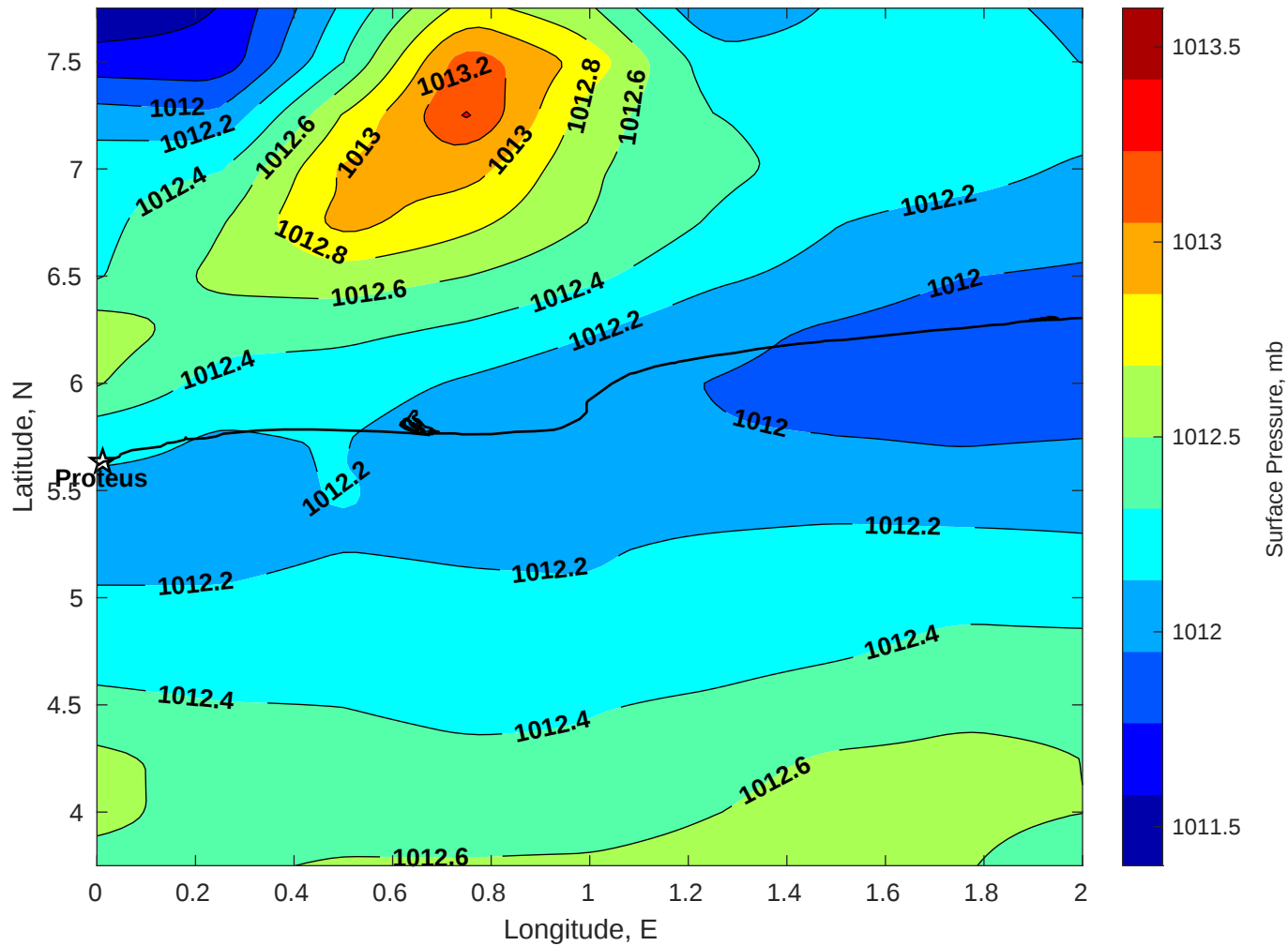
Surface Pressure (mb) for Proteus at 13-Nov-2025 00:00:00
